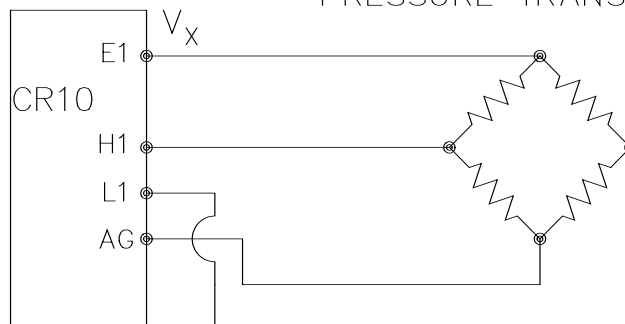
PRESSURE TRANSDUCER
