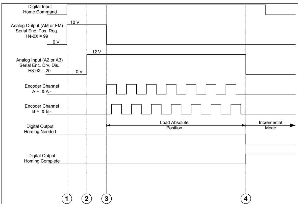
Figure 21: Absolute Incremental Encoder Homing Routine
