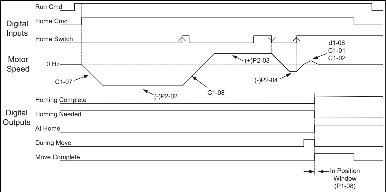
Figure 12: Home Negative with Backup Timing Chart (P2-01 = 1)
