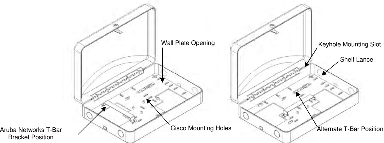
Figure 1 - Model 1016-00 Features
