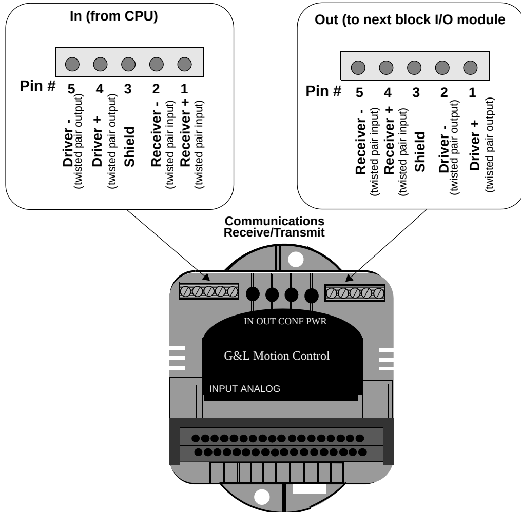
Figure 12-4 Pinouts for Communication Connectors
