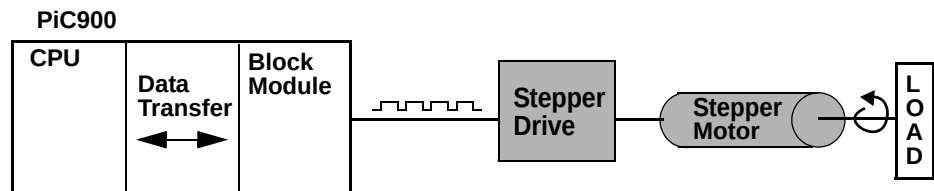
Figure 10-11 Open Loop Stepper System
