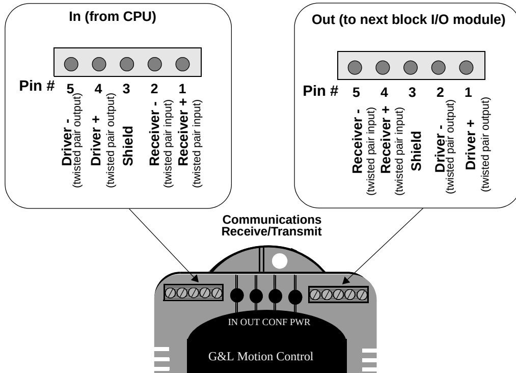
Figure 9-5 Pinouts for Communication Connectors
