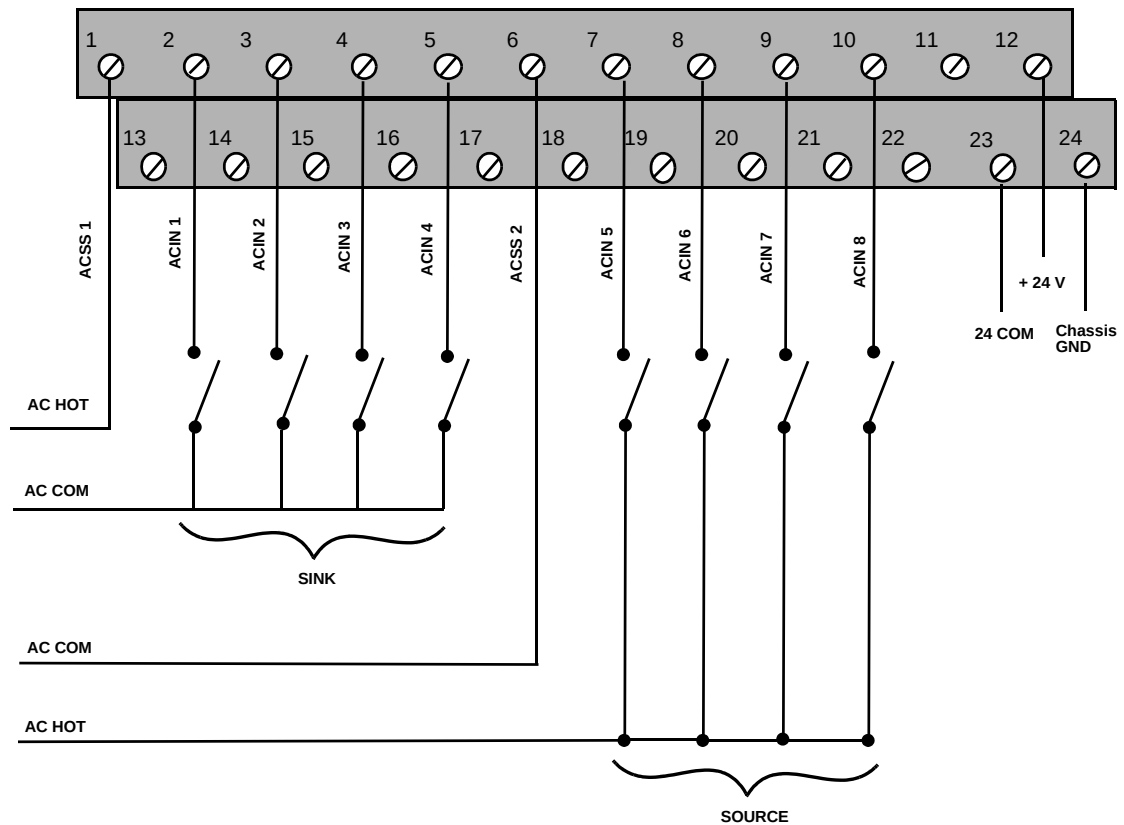
Figure 8-3 Power Connections
