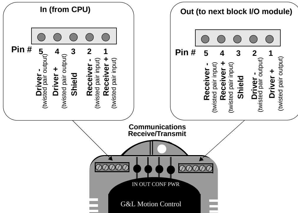
Figure 8-4 Pinouts for Communication Connectors
