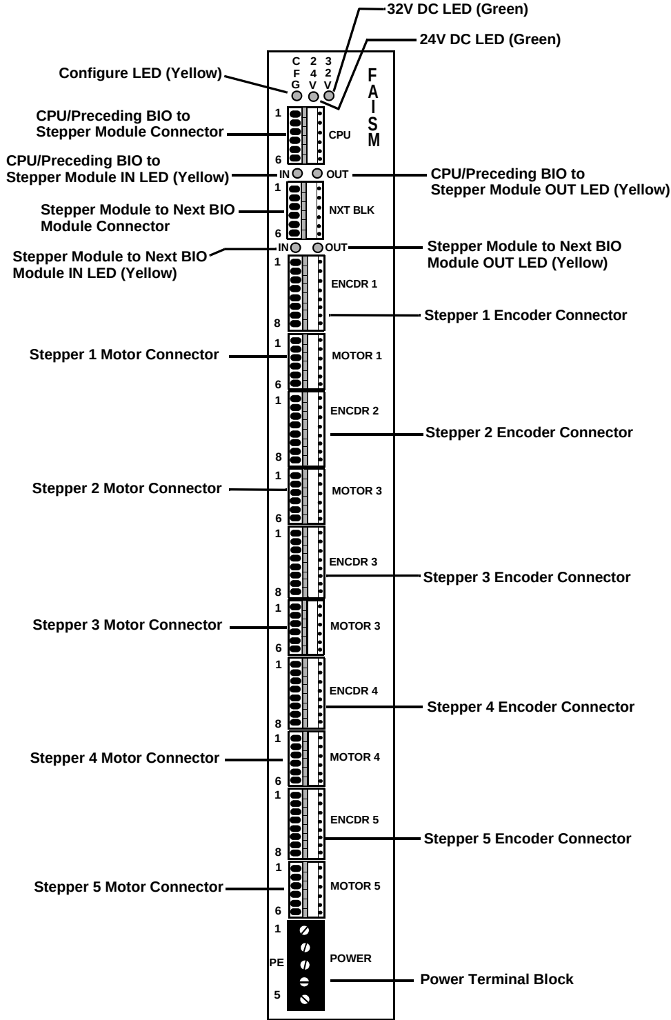
Figure 18-1 5-Axis Integrated Stepper Module
