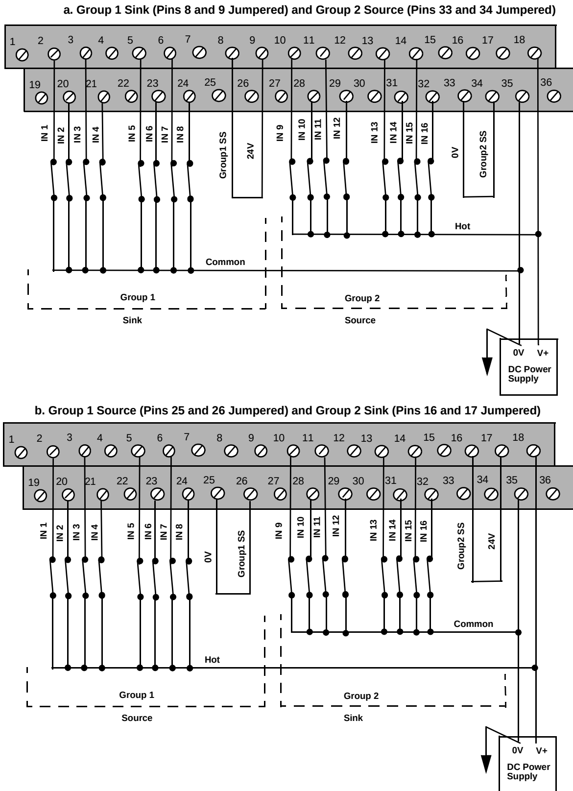
Figure 4-3 Connectors for Two Groups of Inputs
