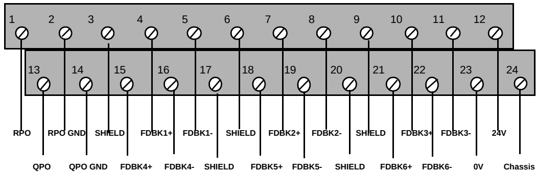
Figure 9-2 Connections for the Block Input Resolver Terminals
