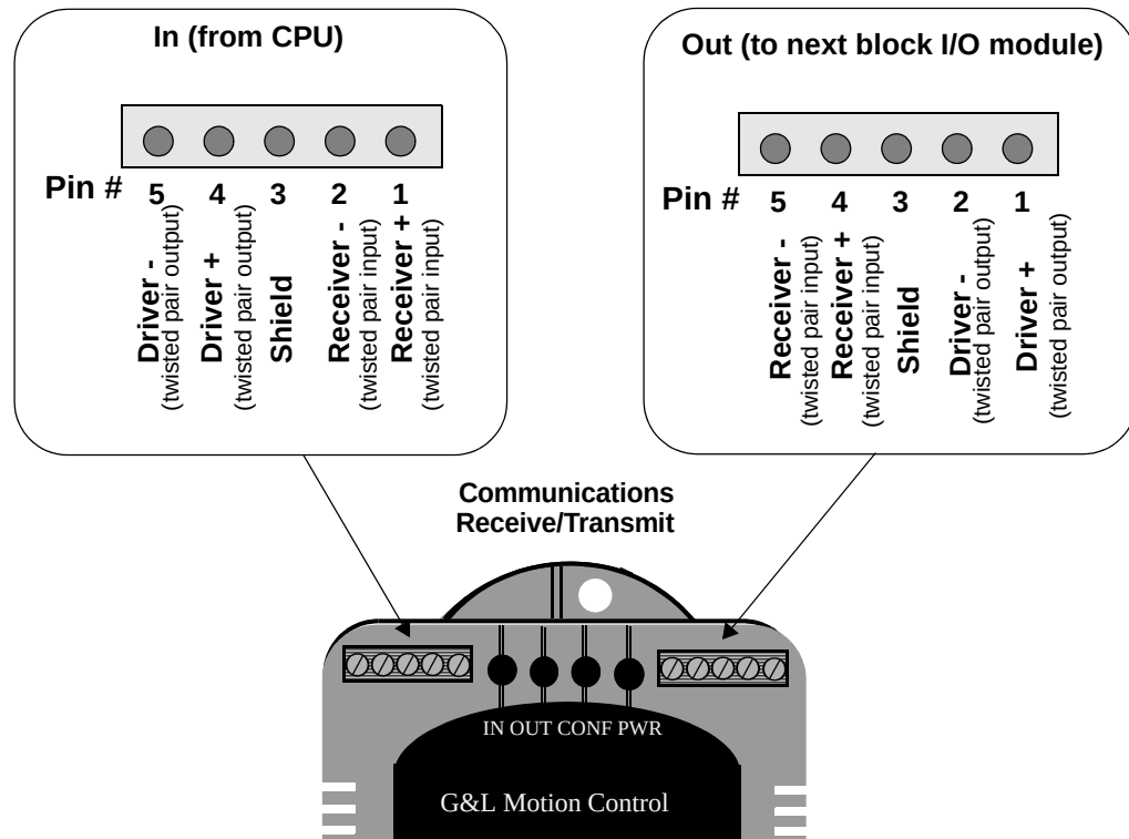
Figure 5-5 Pinouts for Communication Connectors
