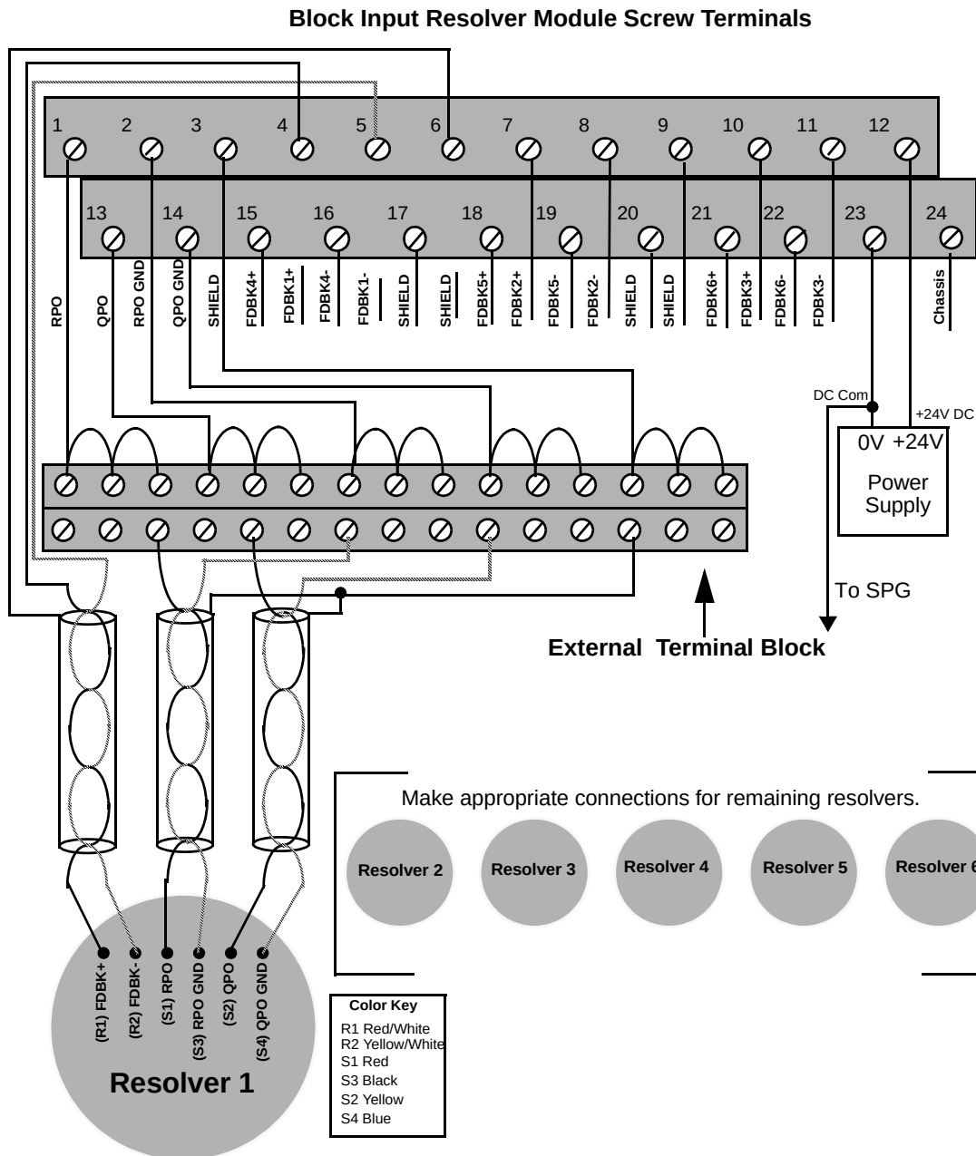
Figure 9-3 Connecting Resolver, Terminal Block, and Module
