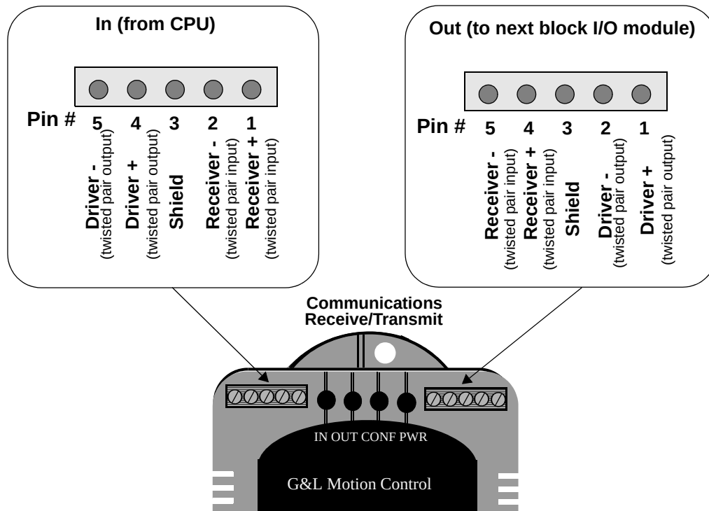
Figure 7-8 Pinouts for Communication Connectors
