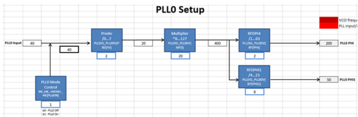
Figure 31. PLL0_PHI configured to 200 MHz
