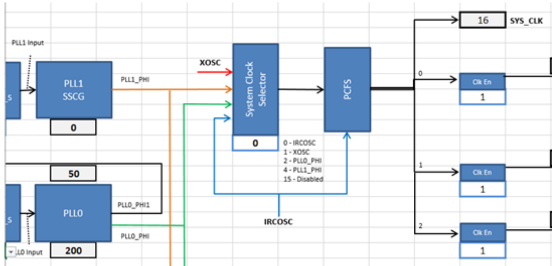
Figure 32. PLL0_PHI propagated to Tree
