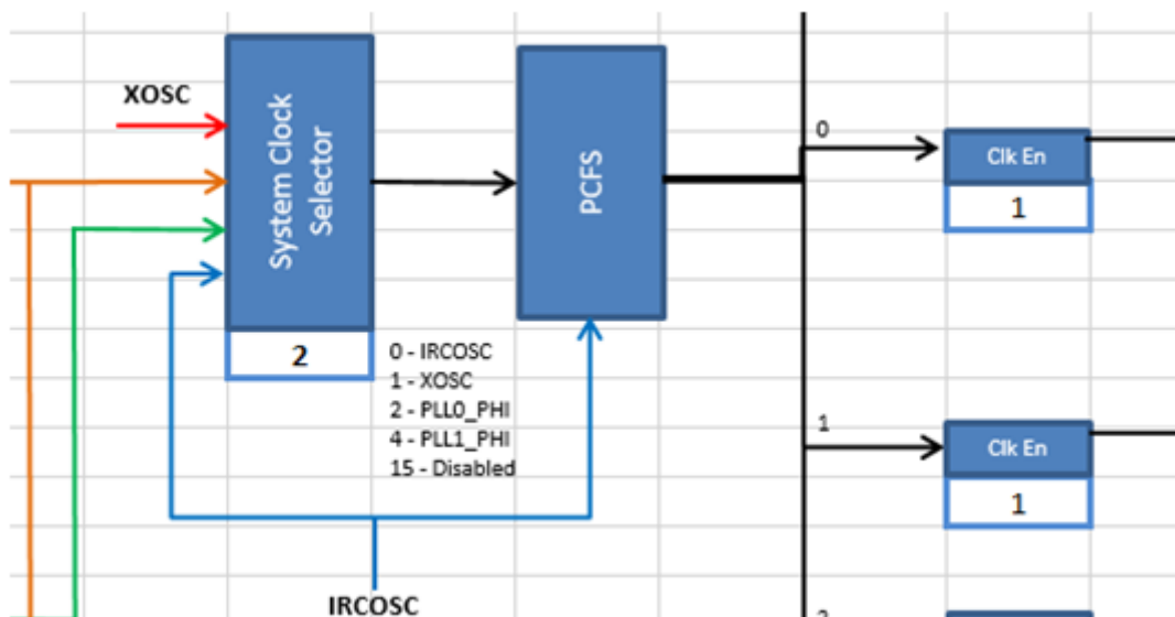
Figure 33. System clock following PLL0_PHI
