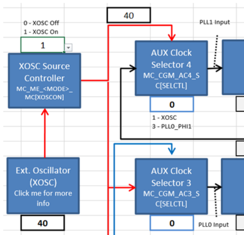
Figure 25. Actual XOSC frequency with source turned on
