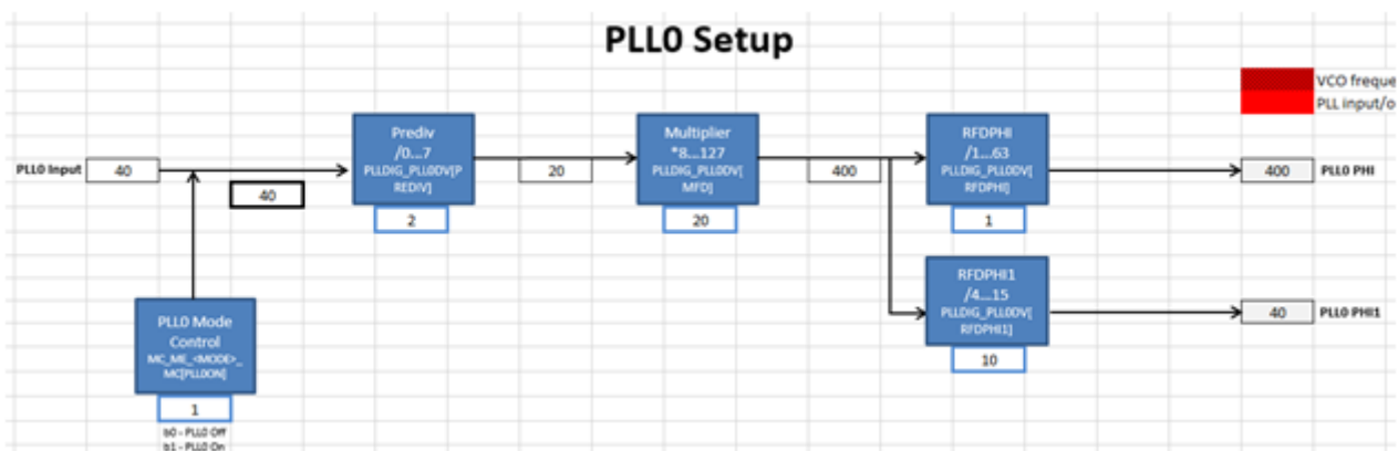
Figure 13. PLL0 control
