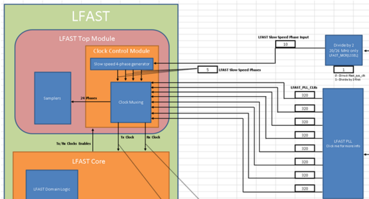
Figure 11. LFAST block diagram
