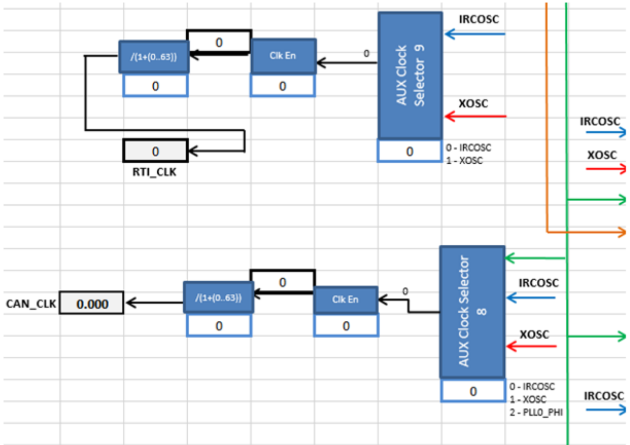
Figure 36. CAN_CLK in Tree
