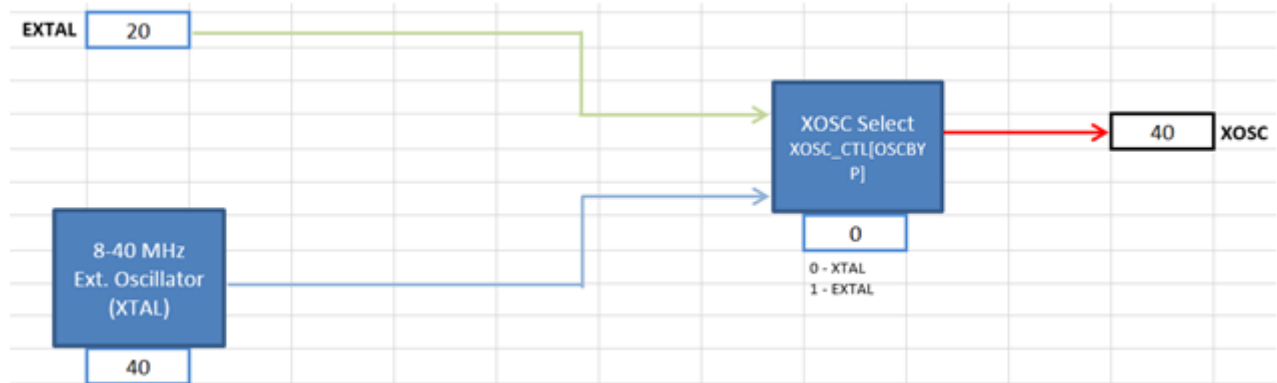
Figure 23. Oscillator configuration
