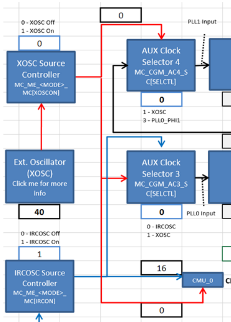
Figure 24. Actual XOSC frequency with source turned off
