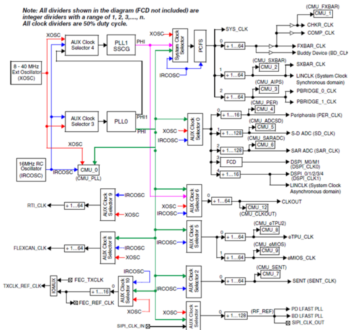
Figure 5. MPC5746R reference manual clock tree
