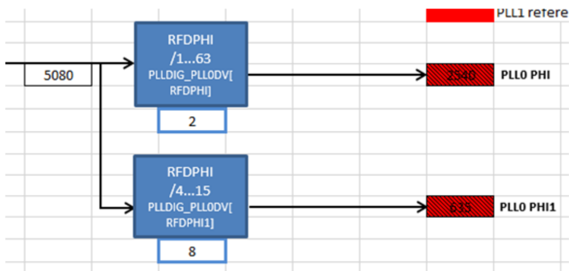
Figure 30. When PLL0_PHI exceeds VCO and PLL spec
