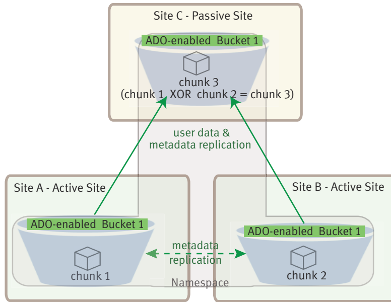
Figure 18 Passive replication in normal state
