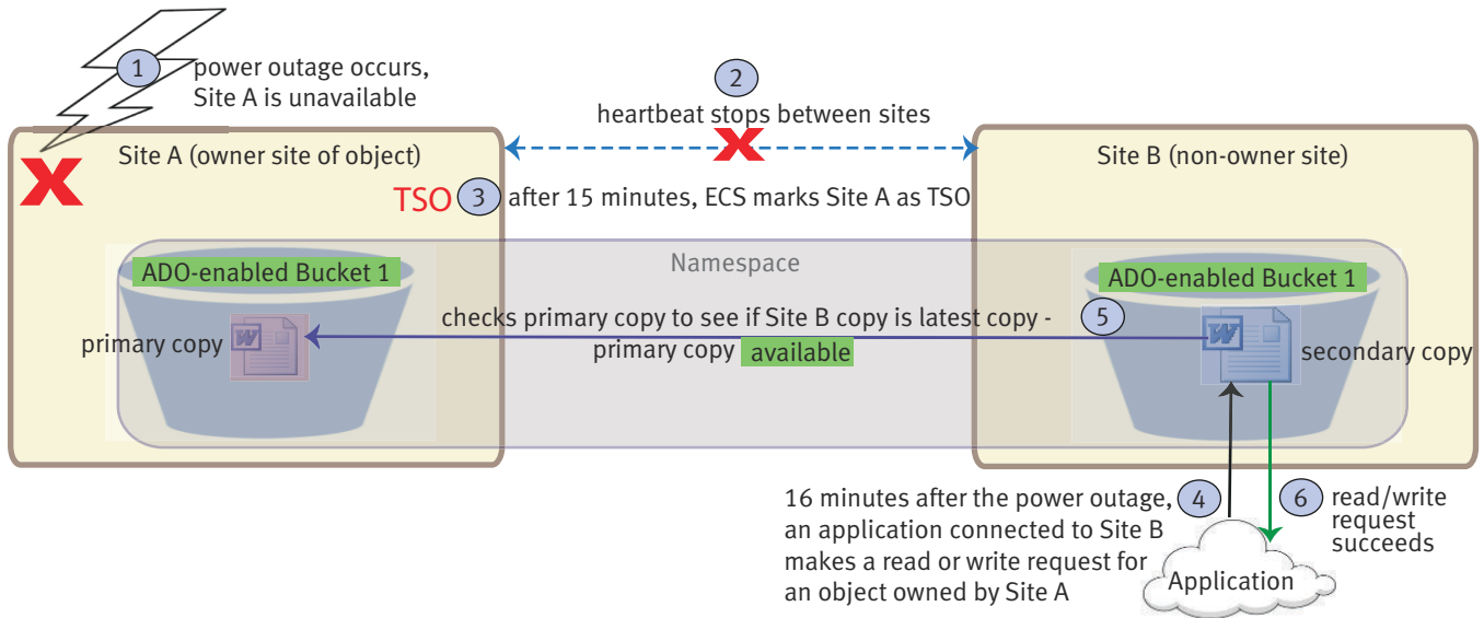
Figure 15 Read/write request succeeds during TSO when ADO-enabled data is accessed from non-owner site and owner site is unavailable
