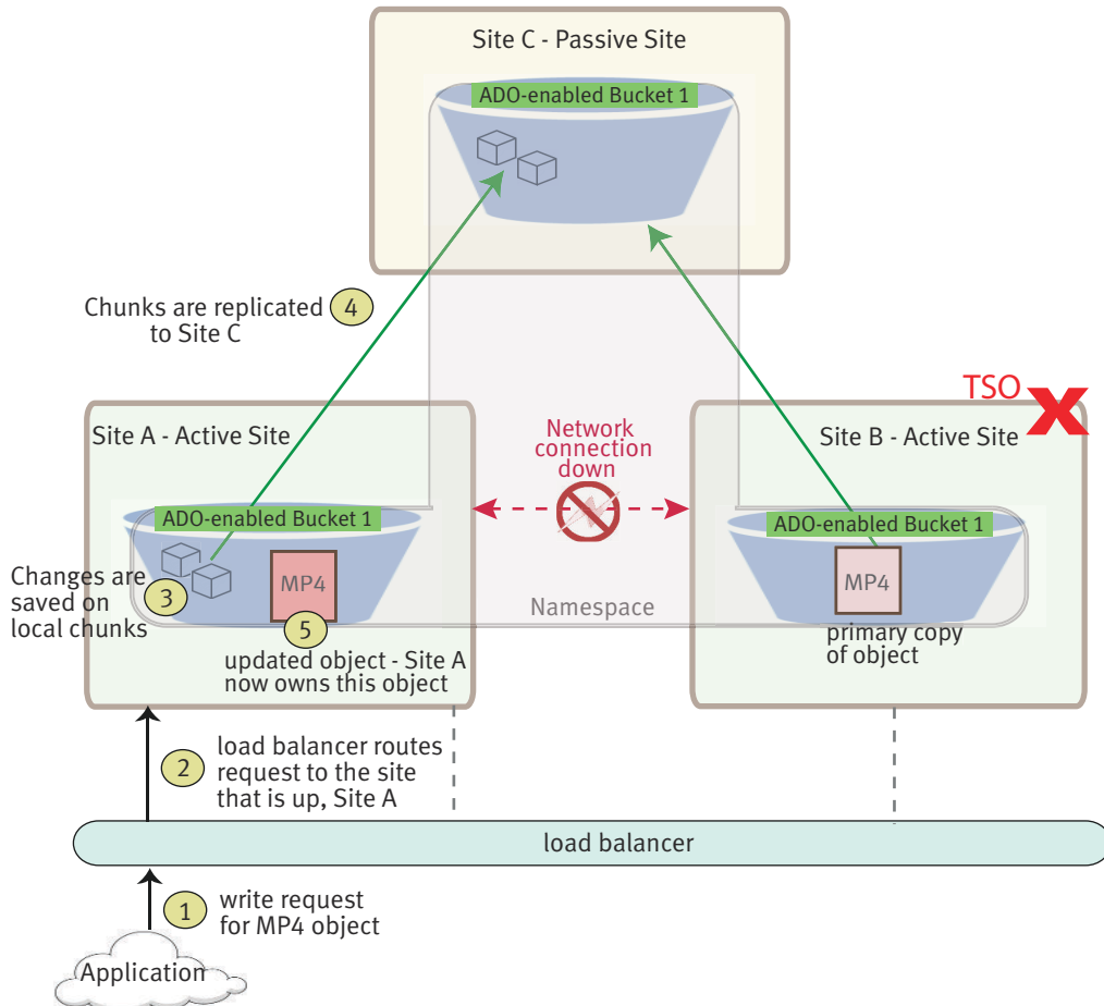
Figure 19 TSO for passive replication
