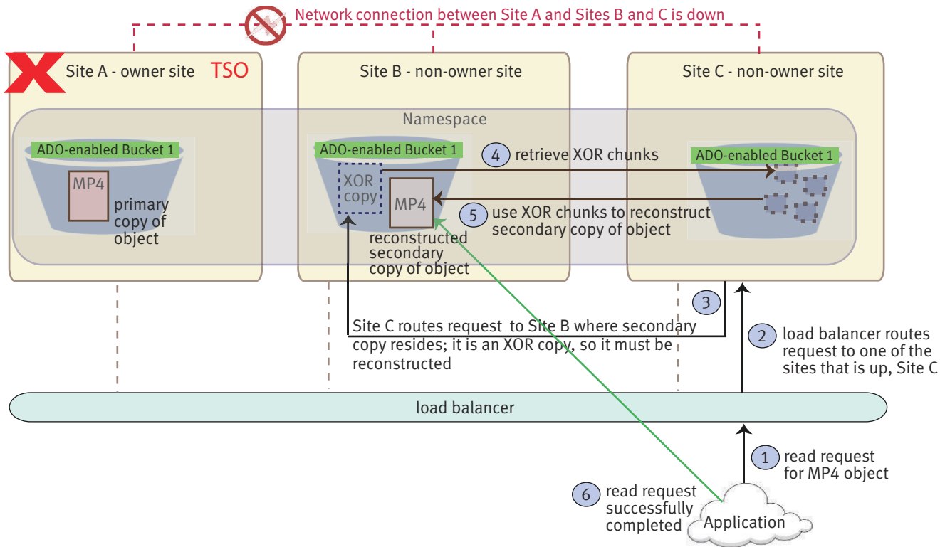
Figure 17 Read request workflow example during a TSO in a three-site federation
