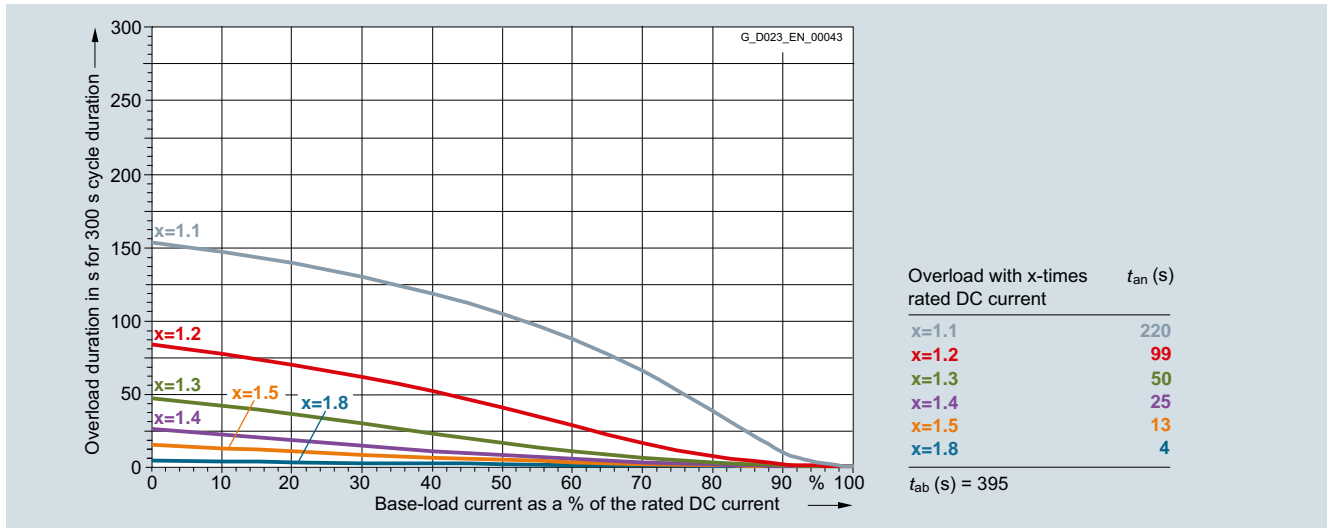
6RA8088-6LS22-0AA0 950 A/two-quadrant operation 830 V, 6RA8088-6LV62-0AA0 950 A/four-quadrant operation 830 V
