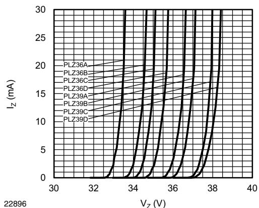
Fig. 11 - Breakdown Characteristics
