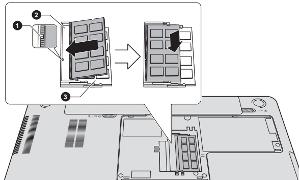
Figure 3-13 Seating the memory module
