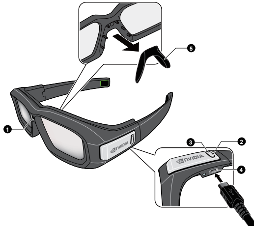
Figure 2-7 3D Vision glass
