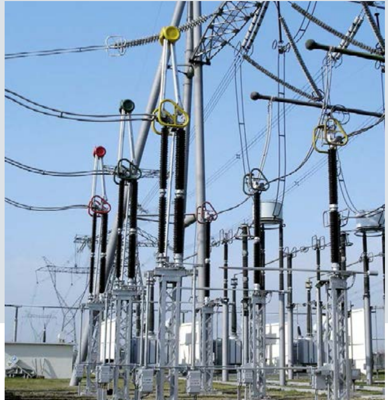
Fig. 29: Knee-type disconnector
