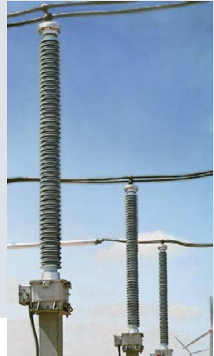
Fig. 52: 245 kV capacitor voltage transformers at Oncor substation (USA)
