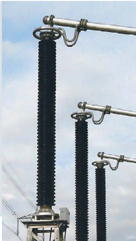
Fig. 55: 420 kV RC dividers (AC) for AIS at Singlewell Substation, National Grid, UK
