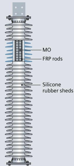
Fig. 37: 3EL-range surge arrester in Cage Design™
