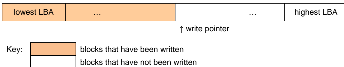
Figure 14 Sequential write required zone and write pointer
