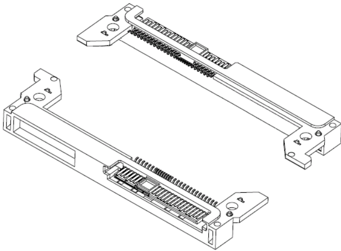
Figure 4 SAS Connector
