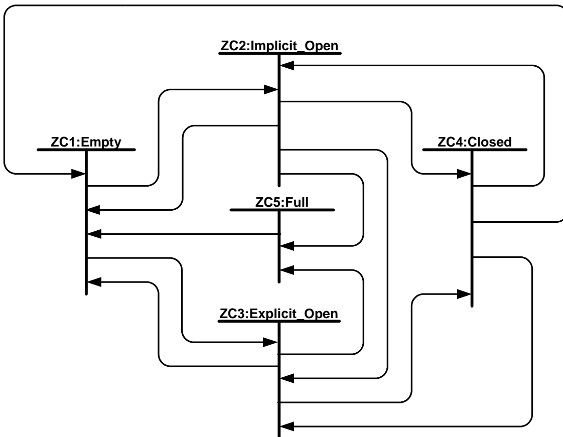
Figure 16 Zone condition state machine
