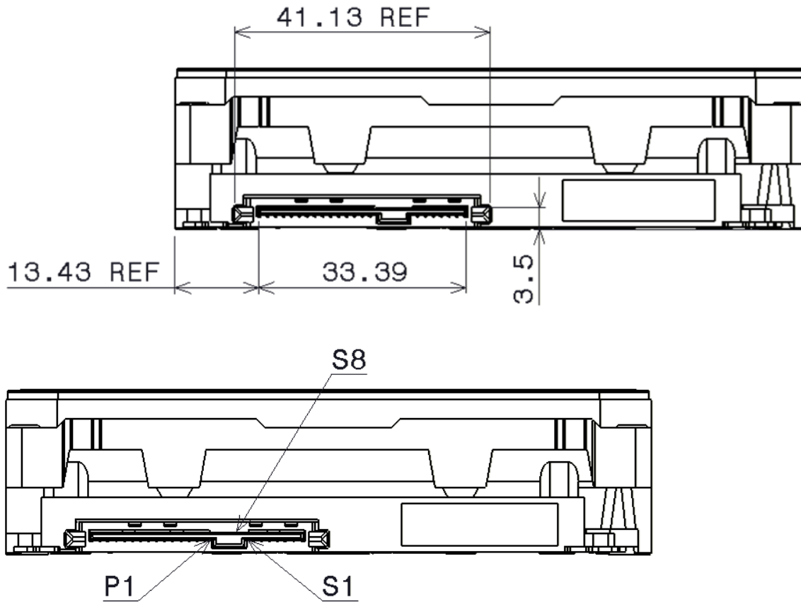
Figure 9 Connector locations
