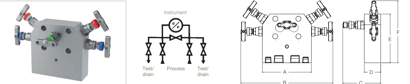
HD*5MCPEXT - Female threaded - NPT x Flanged
