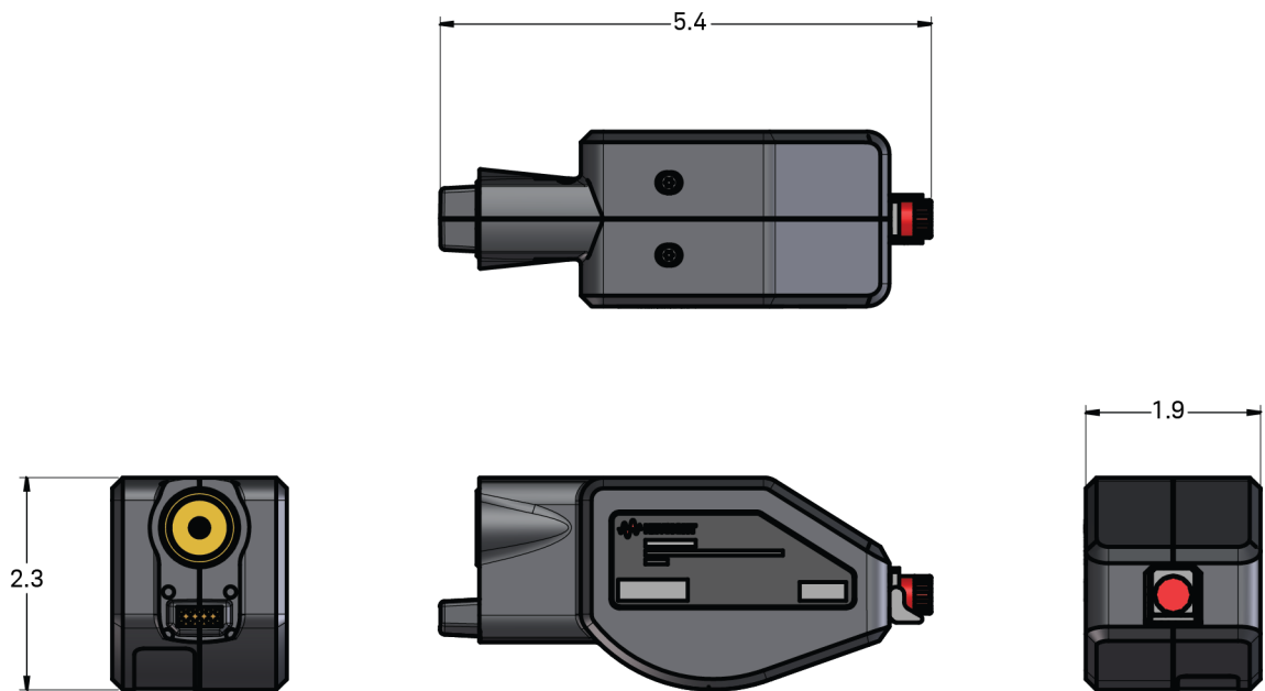
Figure 3 N7004A Dimensions
