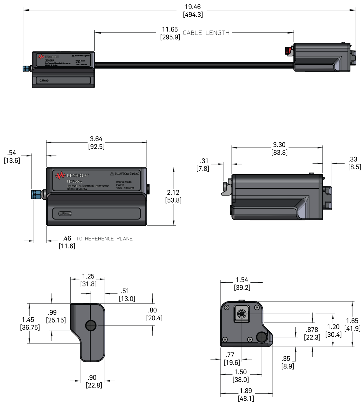
Figure 4 N7005A Dimensions
