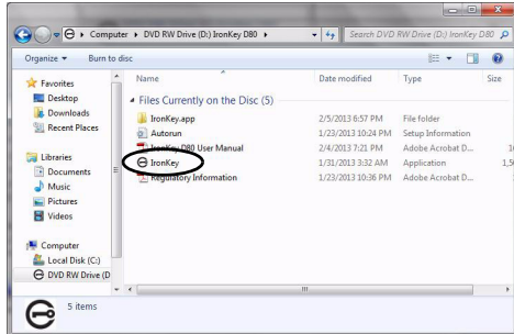
Windows environment
