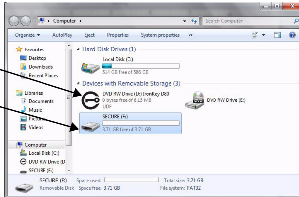
Windows environment
