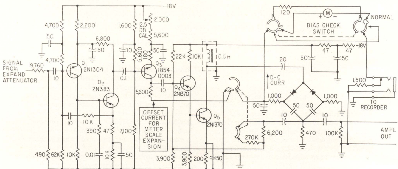
FIG. 2—Schematic of instrument amplifier chain shows derivation of offset current
