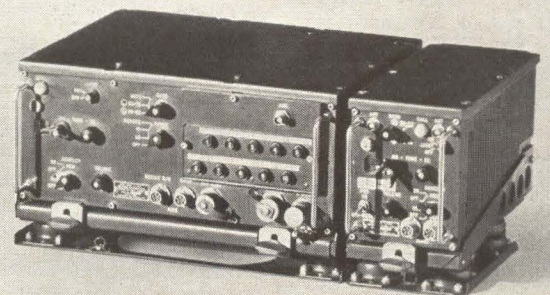
Avco's AN/VRC-12 mobile radio for combat communications
