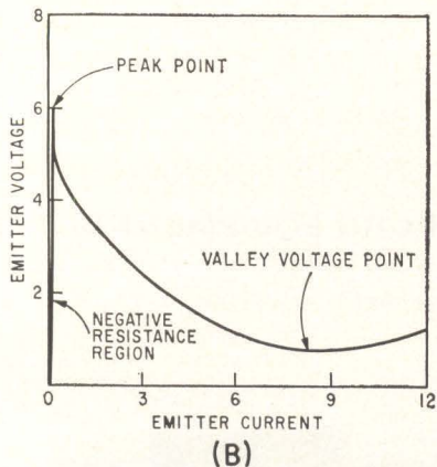
FIG. 1—Equivalent circuit (A) and characteristic curve (B) are shown for unijunction transistor
