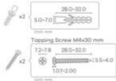
Figure 6 Screw Specifications
