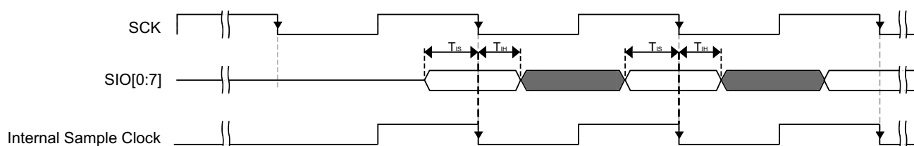
Figure 19. FlexSPI input timing in SDR mode where FlexSPI_MCR0[RXCLKSRC] = 0X0, 0X1
