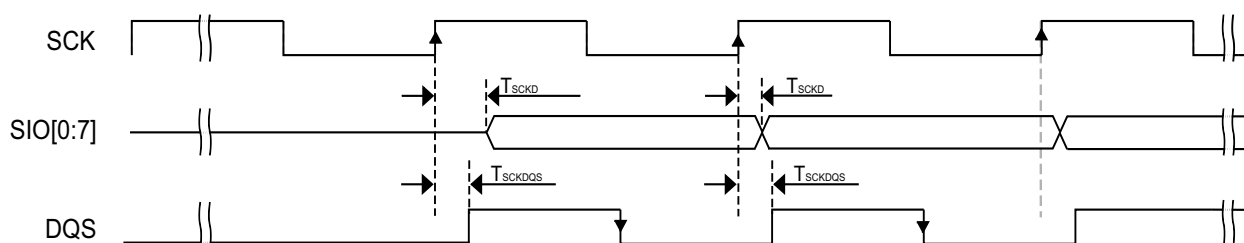
Figure 20. FlexSPI input timing in SDR mode where FlexSPI_MCR0[RXCLKSRC] = 0X3 (Case A1)
