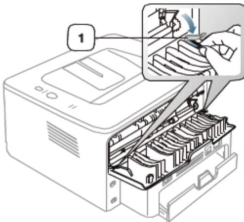
1. Pressure lever
