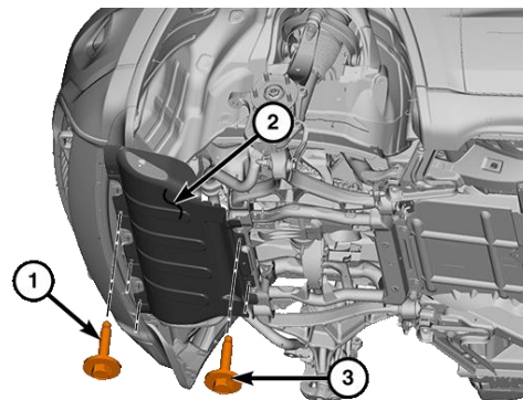
Figure 3 – Front Cover
