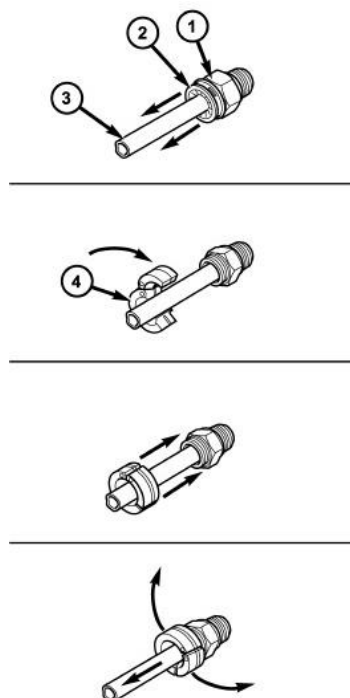
Figure 26 – Quick Connect Fittings
