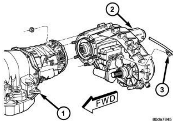
Figure 7 – Transfer Case
