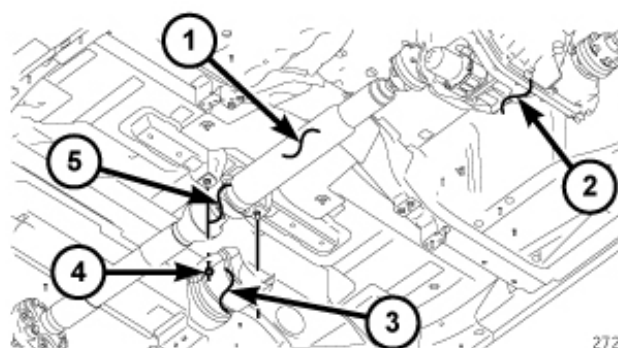
Figure 53 – Heat Shield
