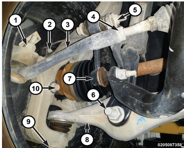
Figure 23 – Clevis Bolt
