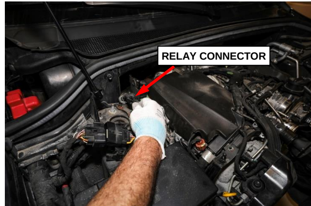
Figure 11 – Relay Connector
