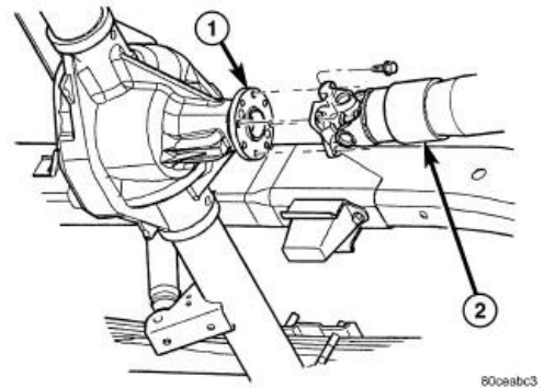
Figure 12 – Pinion Flange
