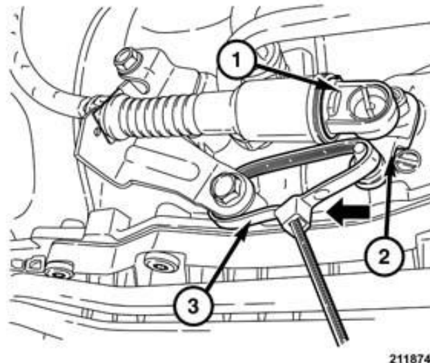
Figure 28 – MPR Cable
