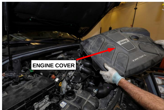
Figure 4 – Engine Cover
