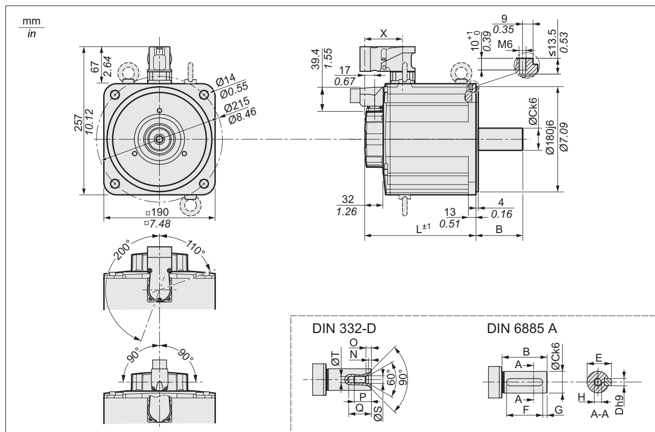
Figure 5: Dimensions MH3190
