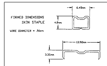
CARTRIDGE CONFIGURATIONS 35 staples
