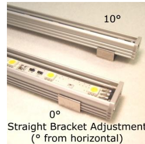
Clip Position
