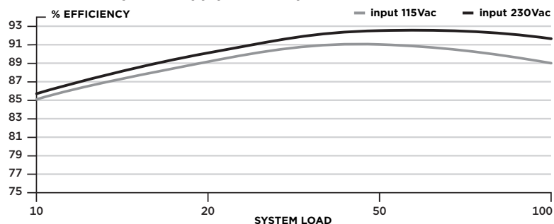
Corsair SF600 power supply efficiency
