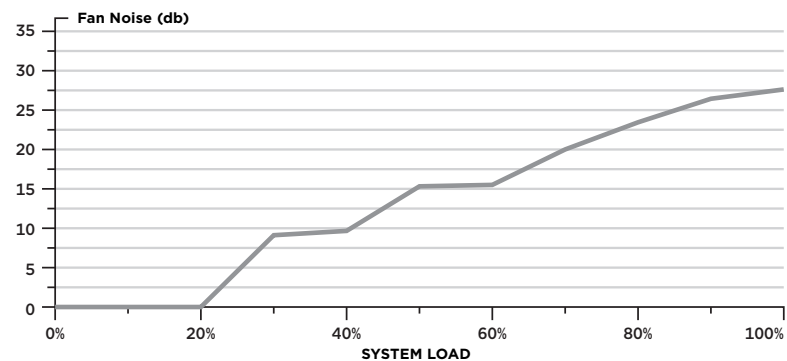
Corsair SF450 power supply fan noise curve
