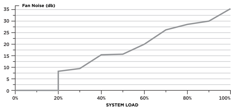
Corsair SF600 power supply fan noise curve
