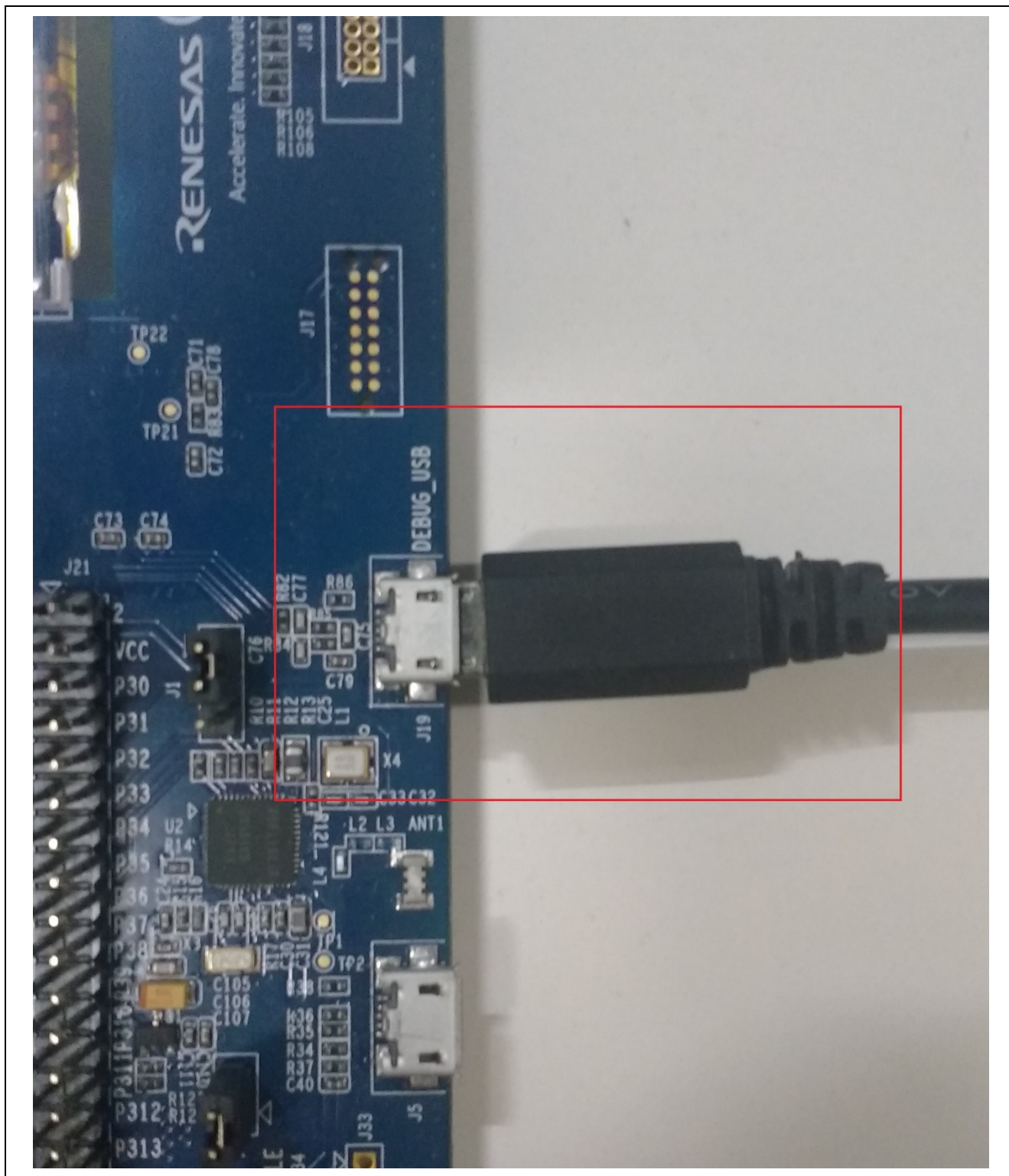
Figure 18 Debug USB
