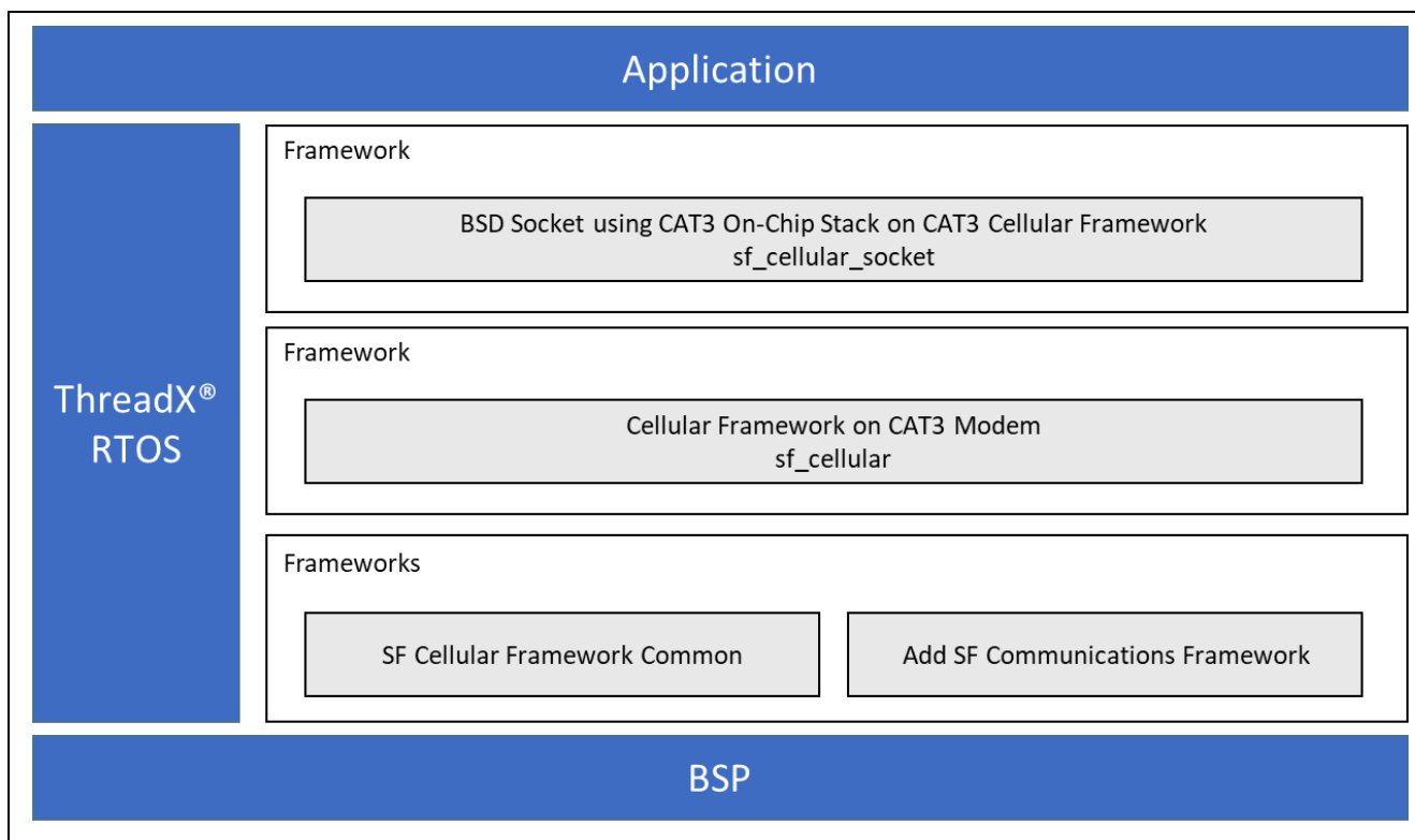
Figure 2 BSD Socket using CAT3 On-Chip Stack on CAT3 Cellular Framework Module Organization, Options, and Stack Implementations
