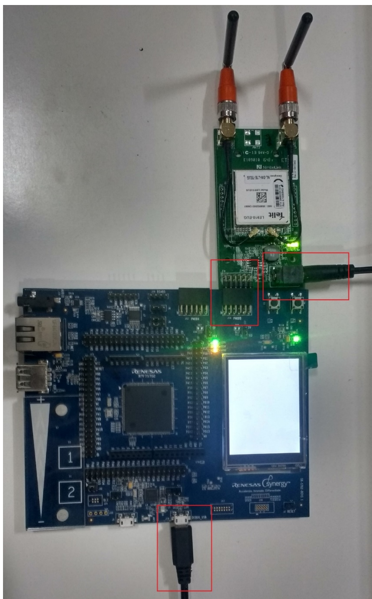
Figure 17 Board Connections
