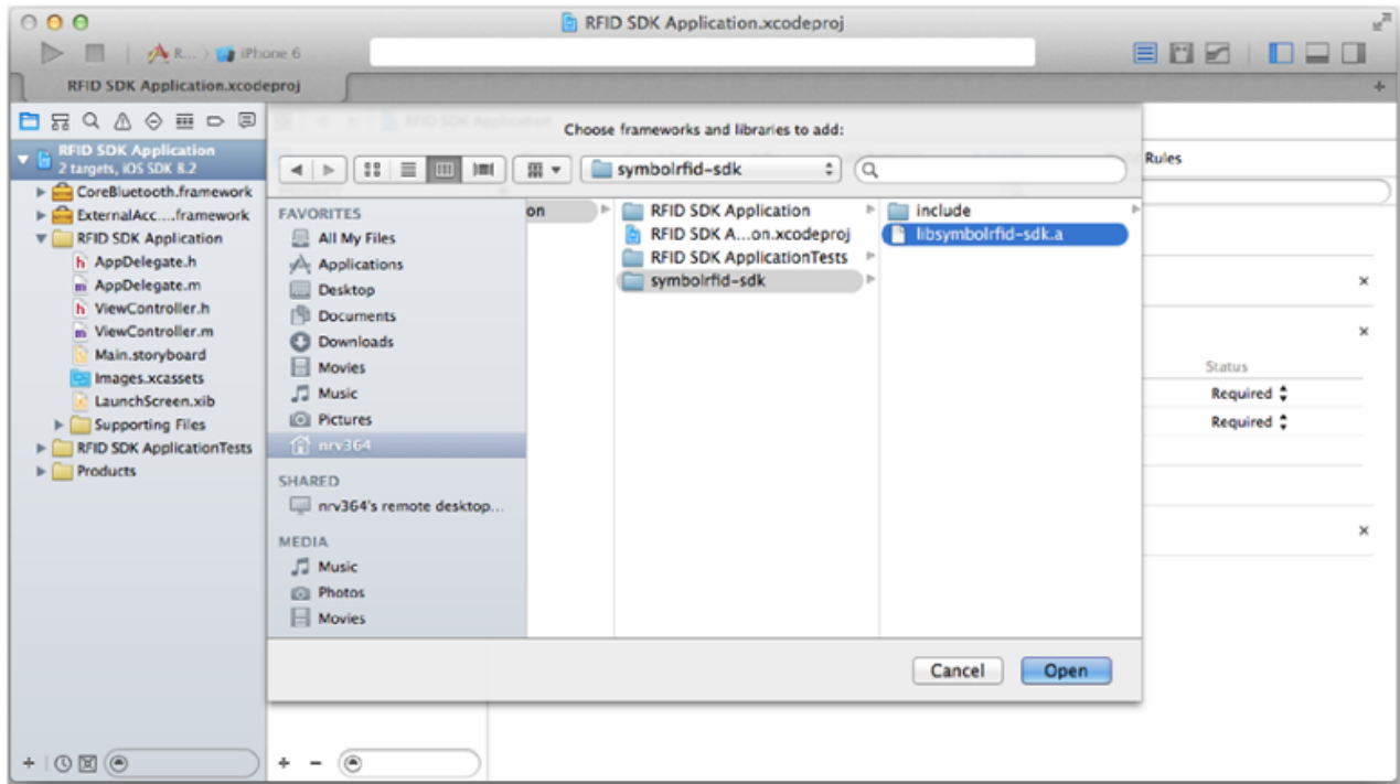
Figure 2-10 Select the Static Library - libsymbolsdk.a
