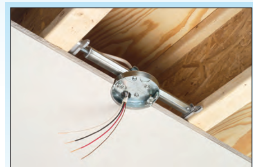
Cut away showing FBR407R installed between wood I-beams
