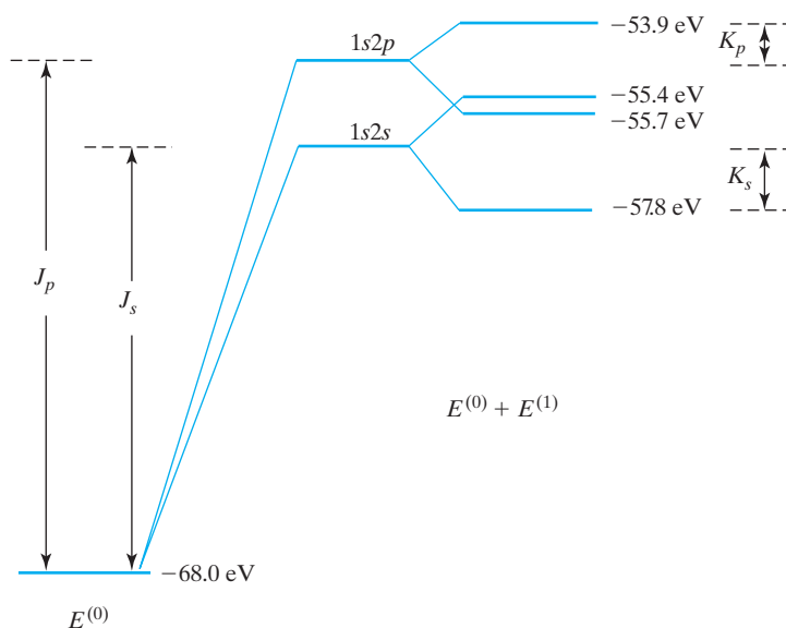
FIGURE 9.3 The first excited levels of the helium atom.
