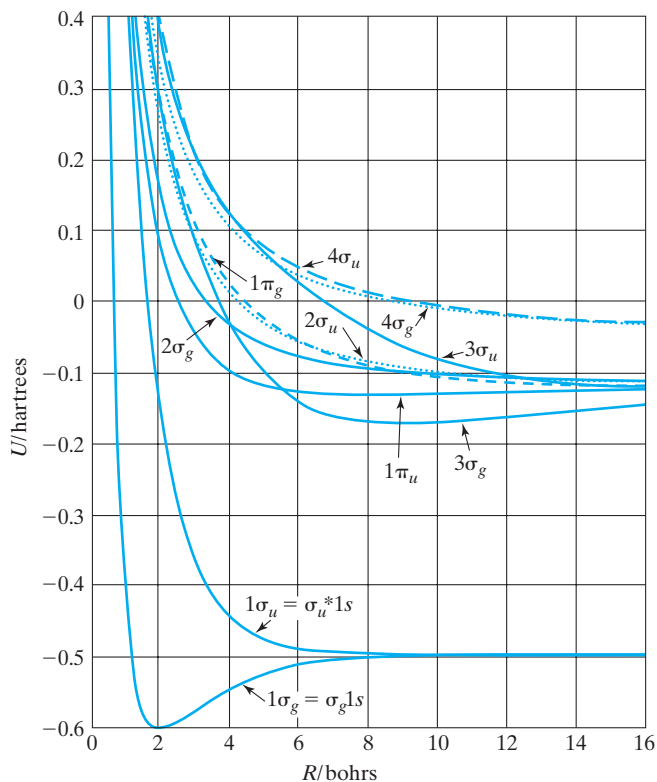
FIGURE 13.5 U(R) curves for several \text{H}_2^+ electronic states. Dashed lines are used to help distinguish closely spaced states. Not visible on the scale of this diagram is a slight minimum in the curve of the first excited electronic state at 12.5 bohrs with a well depth of 0.00006 hartrees.
