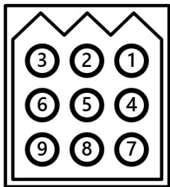
Cabinet Harness 9-pin connector, female
