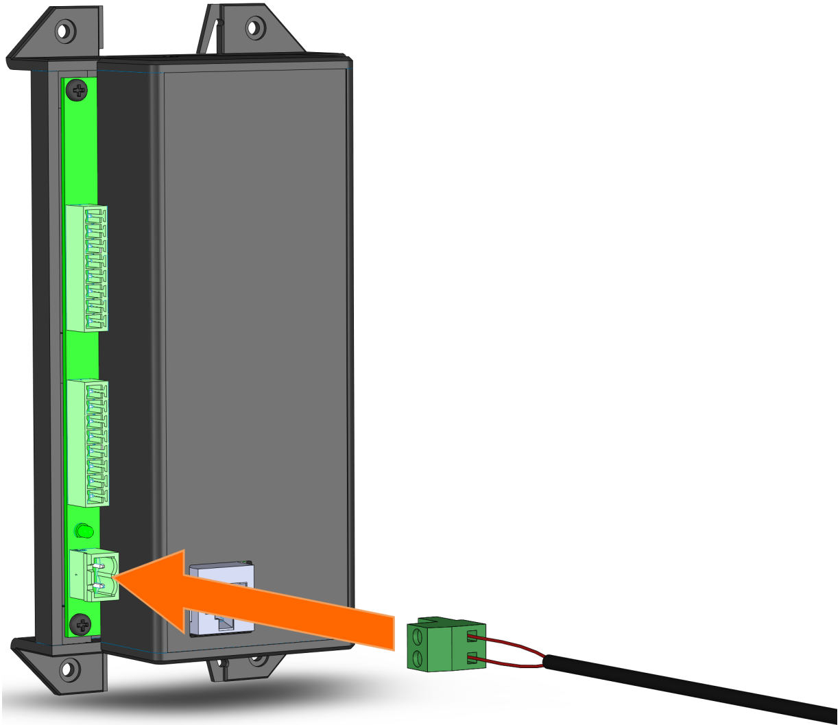
Figure 8 - 1516LI Optional 48VDC Alternate Power Input Connection Example
