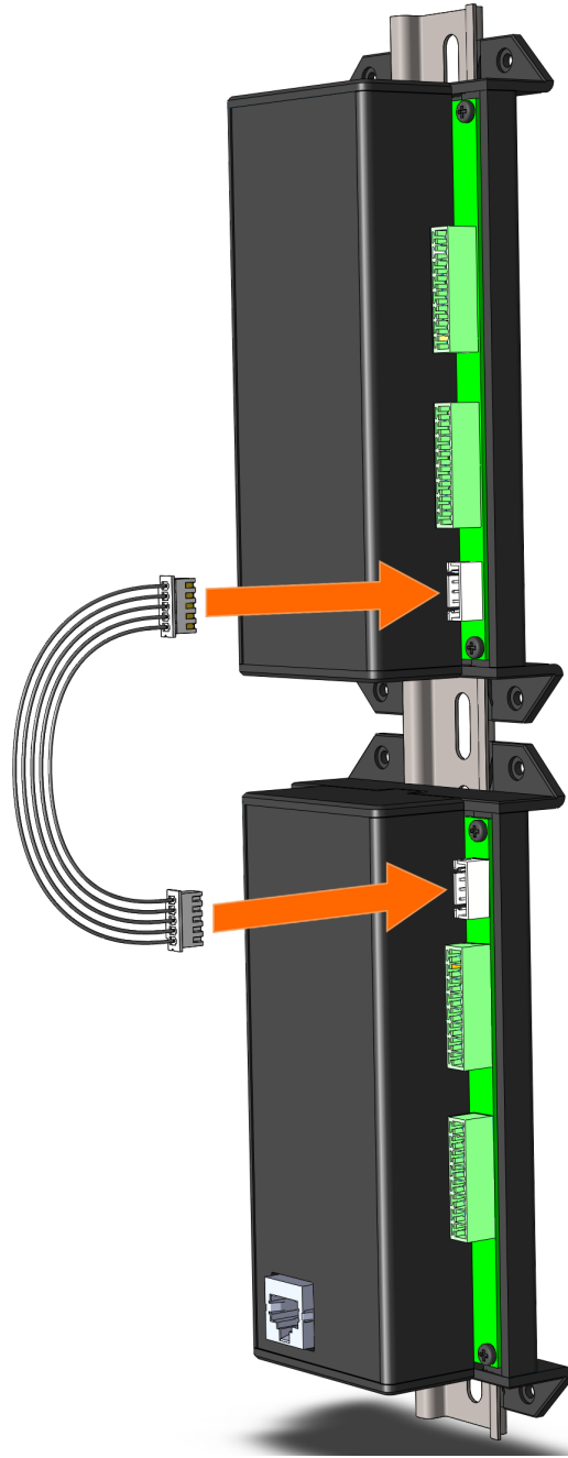
Figure 10 - 1516LI TO 1516LI-E Expansion Bus Connection Example
