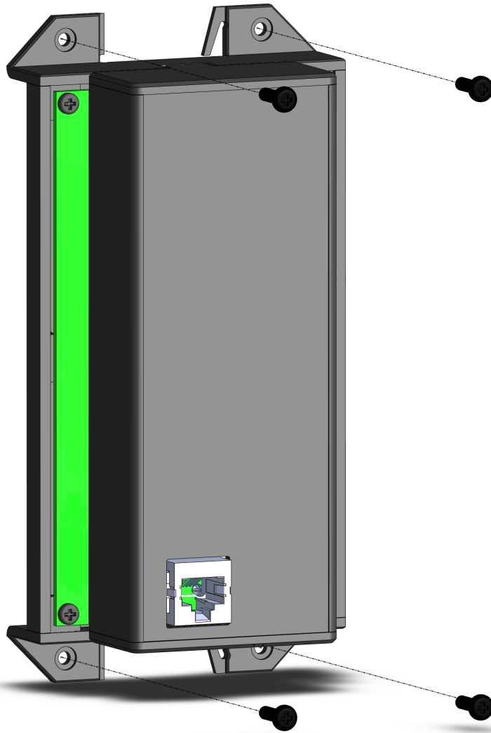
Figure 2 - Wall Mounting with Screws
