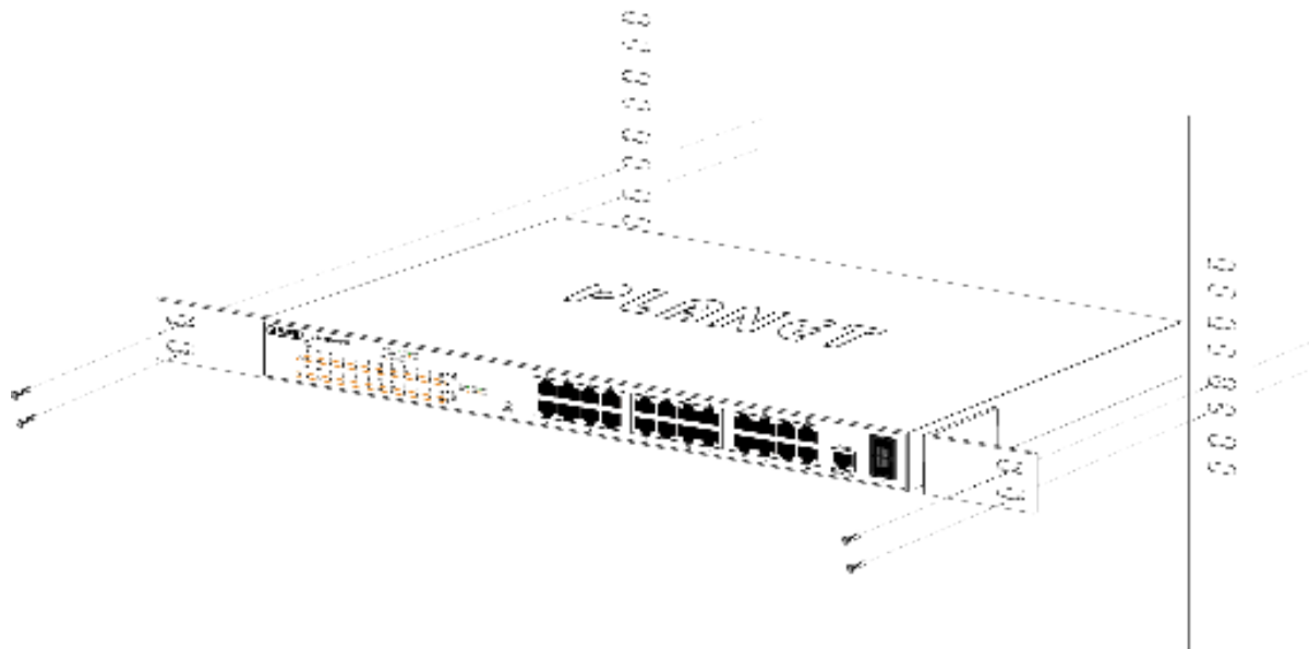
Figure 2-1-11: Mounting Managed Switch in a Rack
