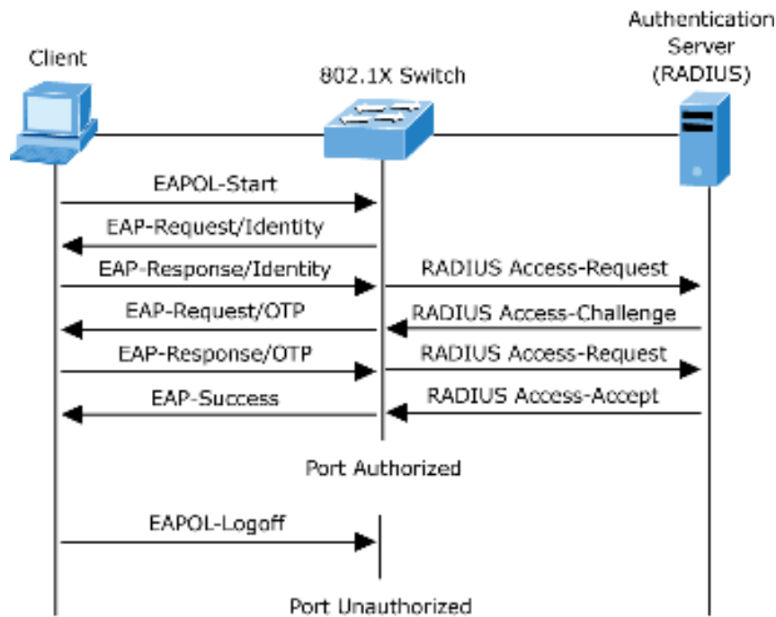
Figure 4-9-6: EAP Message Exchange
