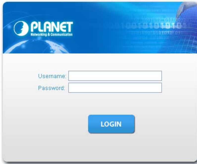
Figure 4-1-2: Login Screen
