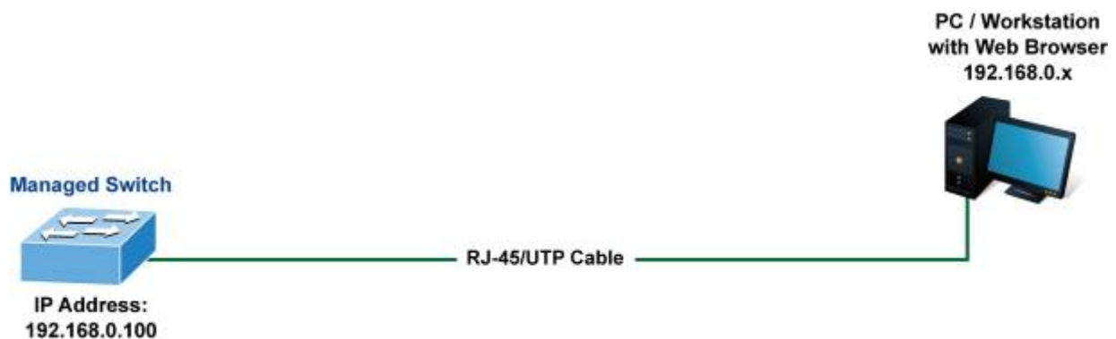
Figure 3-3: Web Management
