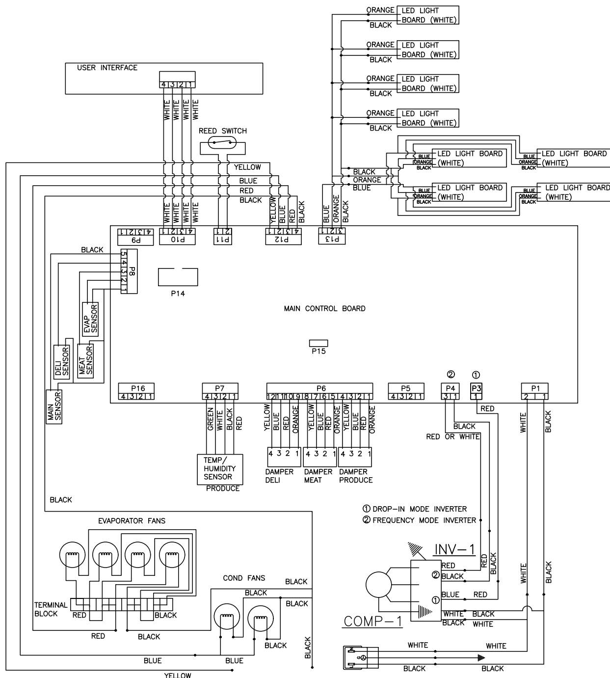
Figure 5-1.1. Refrigerator Column Wiring Diagram
