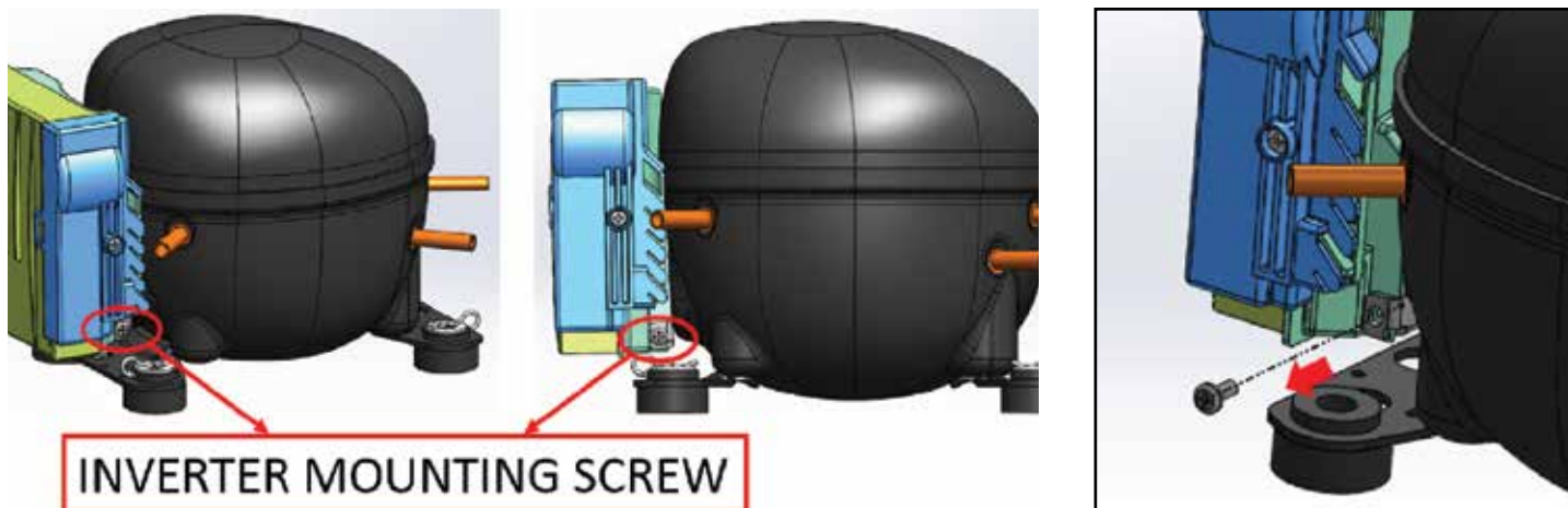
Figure 6-15.3. Inverter Mounting Screw/Electrical Connections
