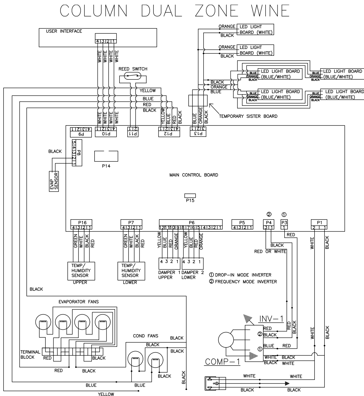
Figure 5-1.3. Wine Column Dual-Zone Wiring Diagram
