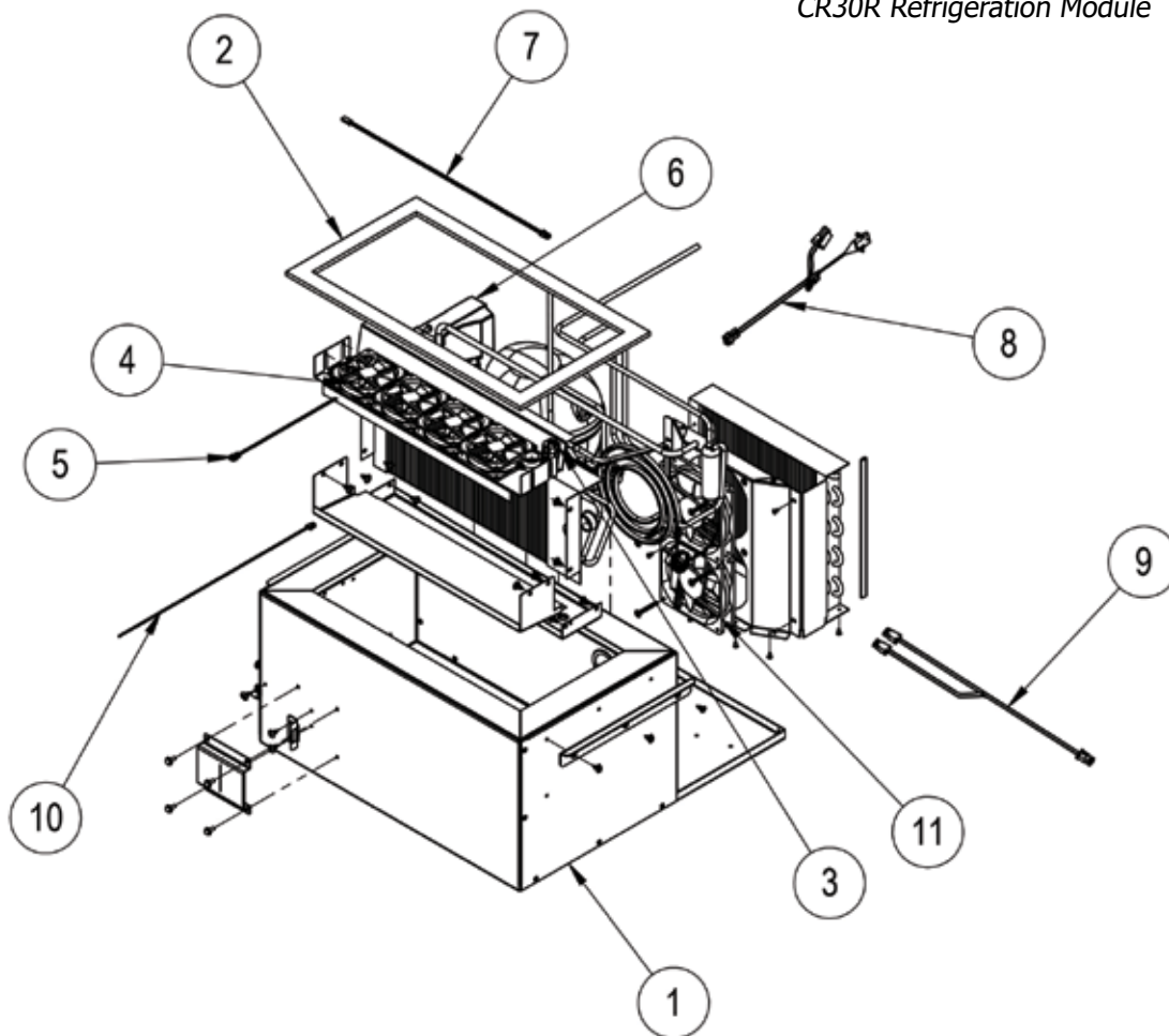
Figure 9-1. CR24R, CR24D, CR24W, CC24D, CC24W, and CR30R Refrigeration Module
