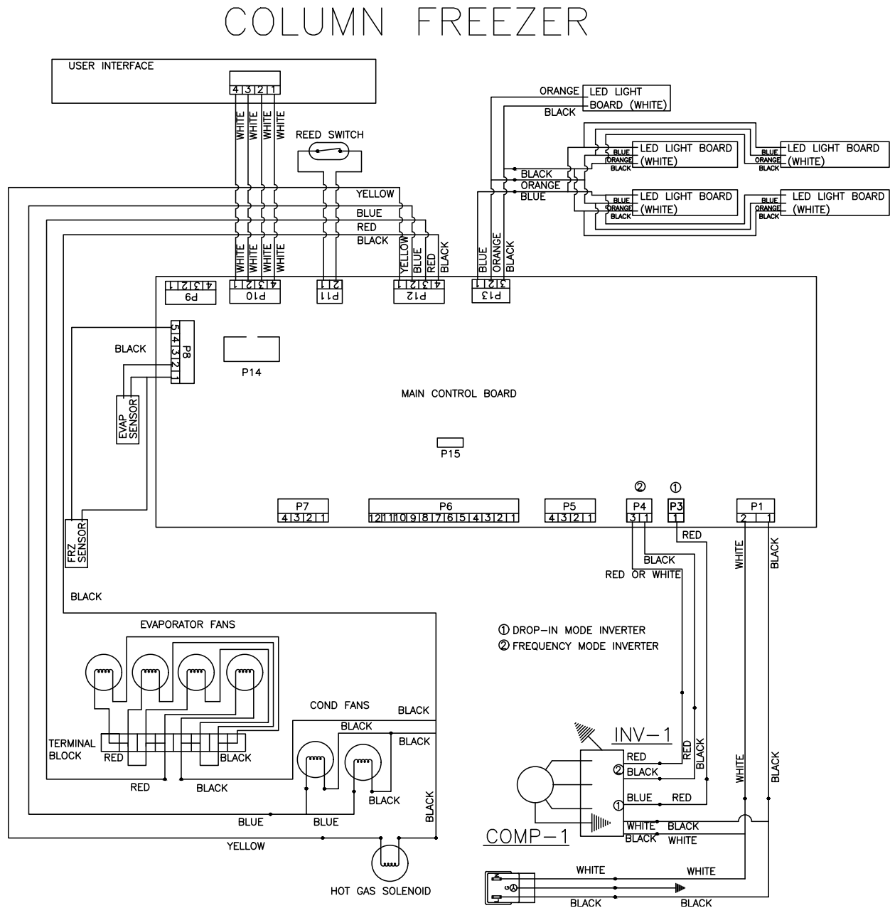
Figure 5-1.4. Freezer Column Wiring Diagram
