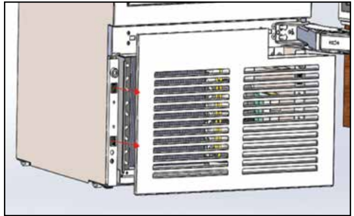
Figure 6-7.1. Remove Grill
