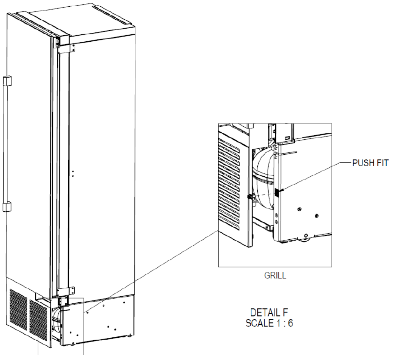
Figure 8-4. Grill Installation
