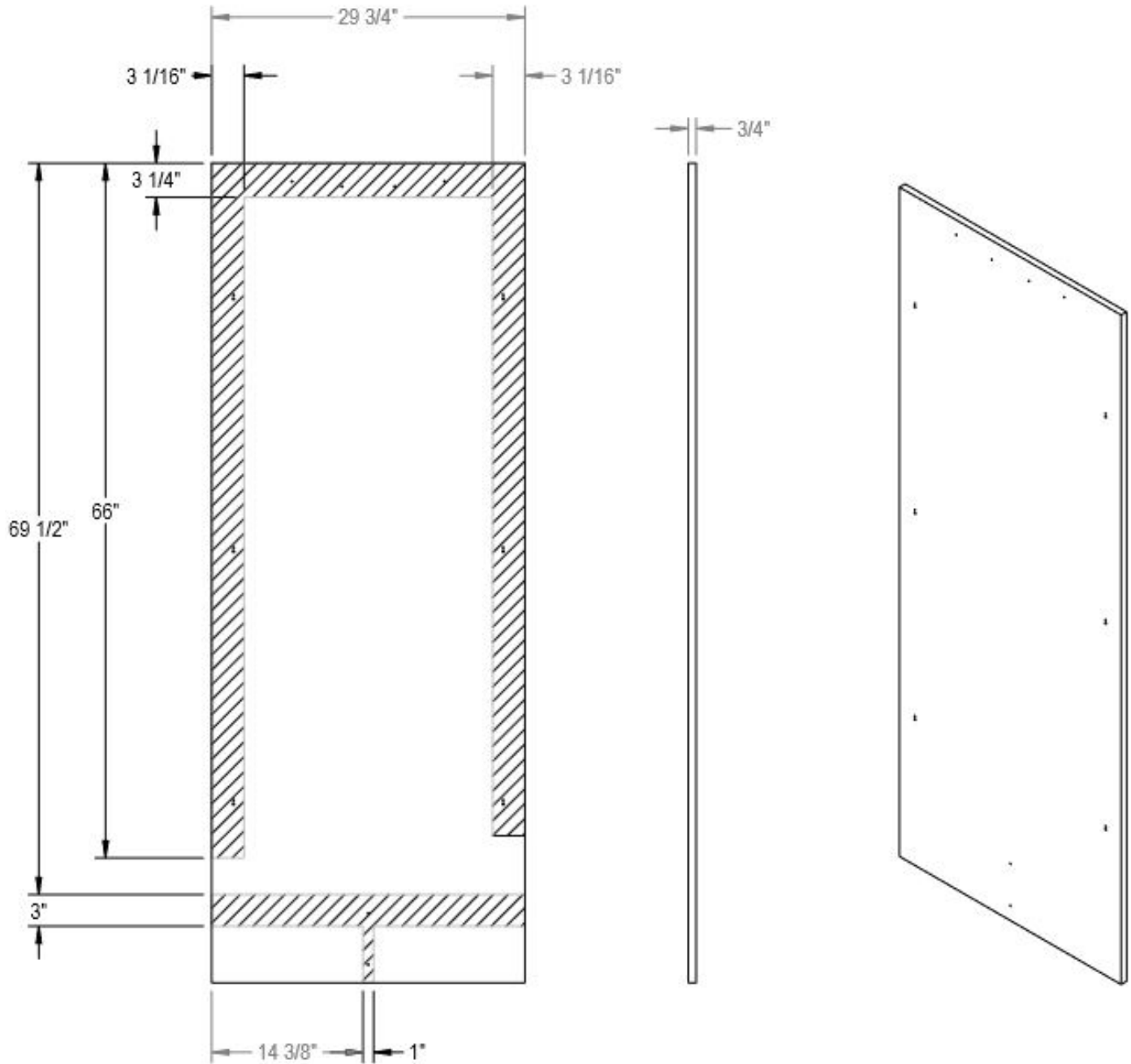
Figure 8-12.2. CR30 Screw Zone For Overlay Templates
