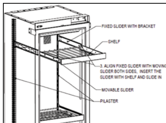
Figure 8-17.4. Install Wine Shelves
