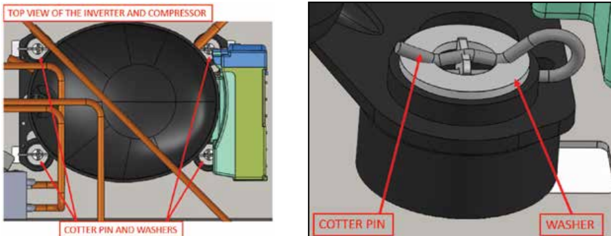
Figure 6-15.1. Remove Cotter Pins
