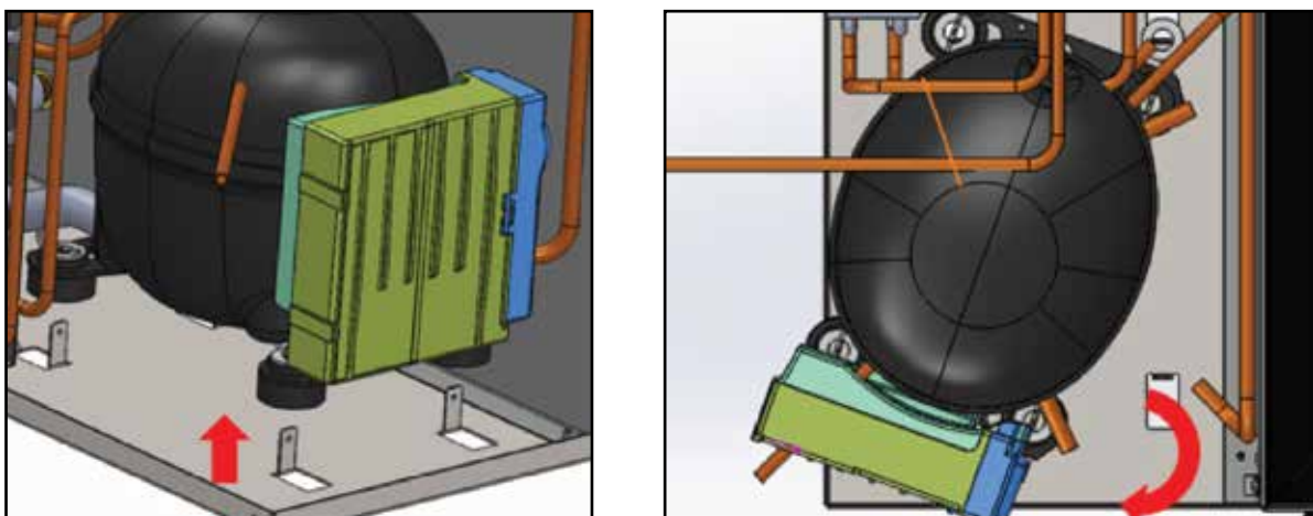
Figure 6-15.2. Lift And Rotate Compressor
