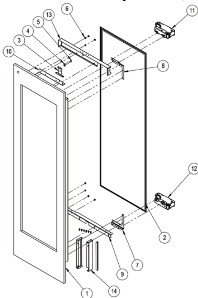
Figure 9-11. CR24D, CR24W, CC24D and CC24W Door
