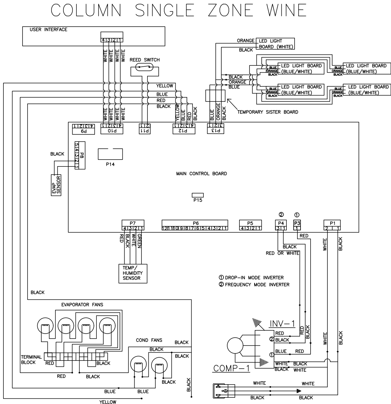
Figure 5-1.2. Wine Column Single Zone Wiring Diagram
