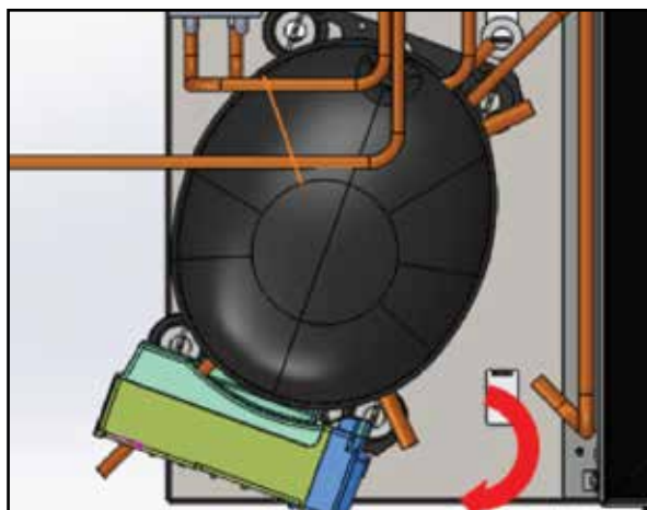
Figure 6-15.4. Lift Inverter
