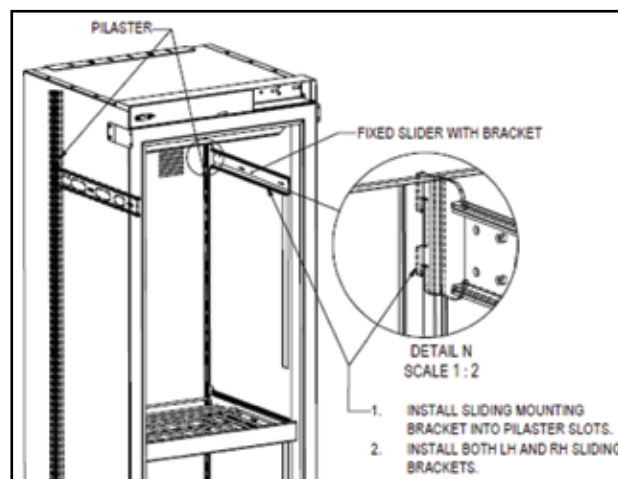
Figure 8-17.3. Install Wine Shelves
