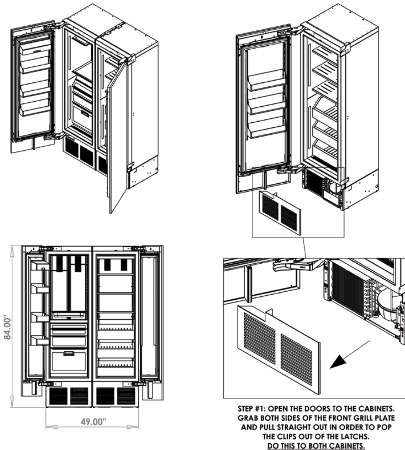
Figure 8-23.1. Marriage Kit Install (1)
