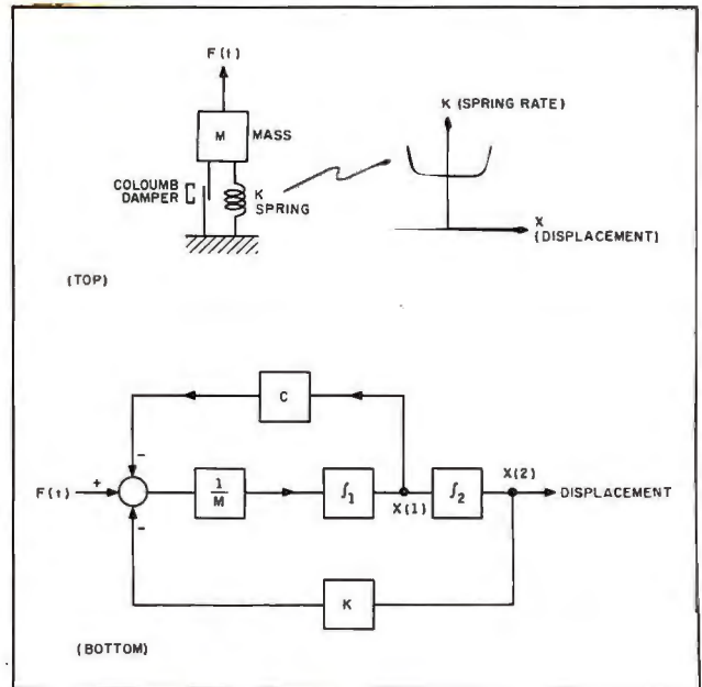
Figure A: The top of this figure shows a mechanical model of a damped spring-mass system. The bottom shows a block diagram of an analog model equivalent to the mechanical model.
