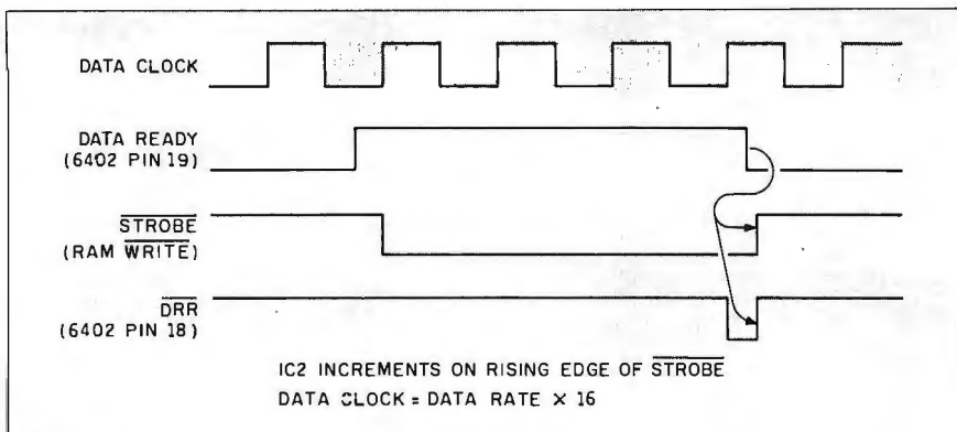
Figure 2: RAM load timing.
