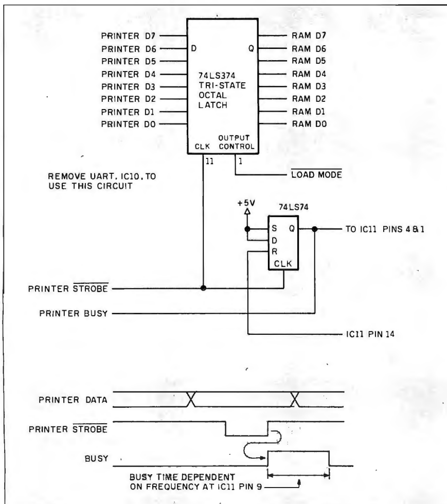
Figure 3: Schematic for interfacing the Emulo-8 to a printer port with the load timing using the printer interface.
