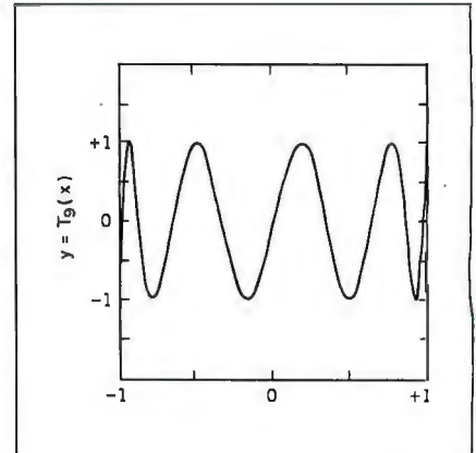
Figure 7: The Chebyshev polynomial of degree 9.
