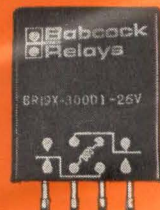
BR-19—Subminiature all-welded 10 amp relay. BR-20 magnetic latching version also available.
