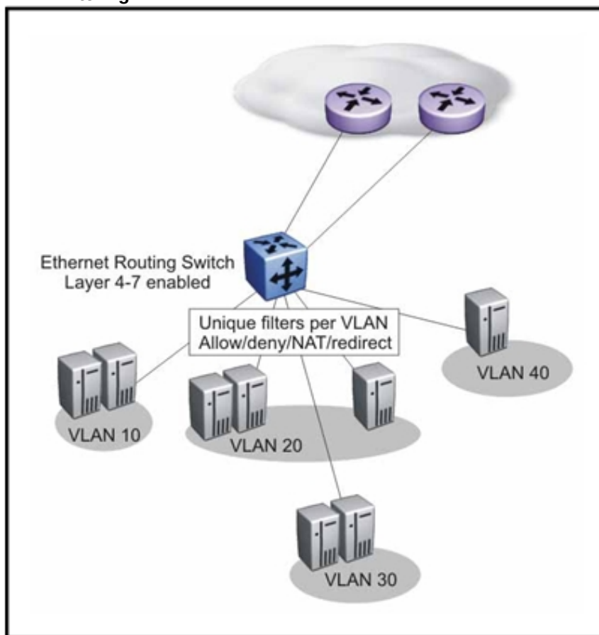
Figure 126 VLAN filtering
