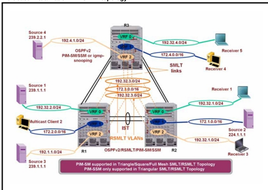
Multicast virtualization in RSMLT topology
