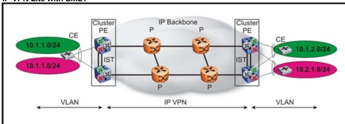
Figure 106 IP VPN Lite with SMLT
