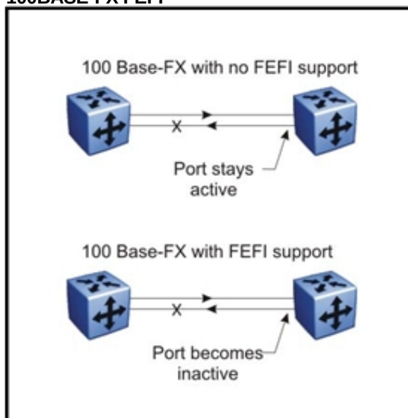
Figure 13 100BASE-FX FEFI
