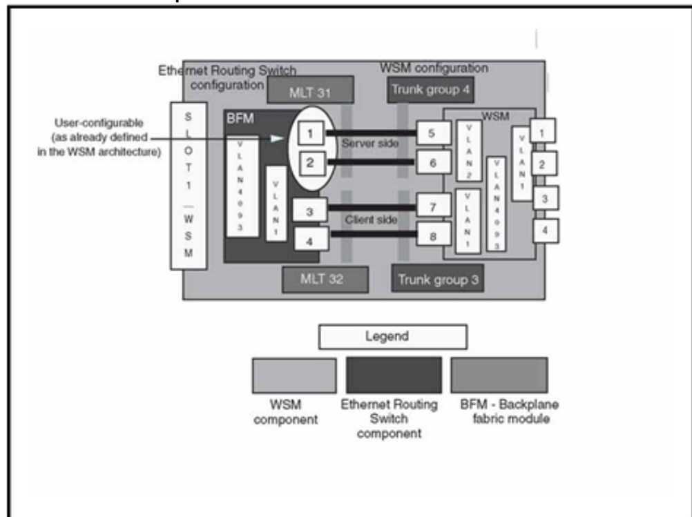
Figure 125 Detailed WSM data path architecture
