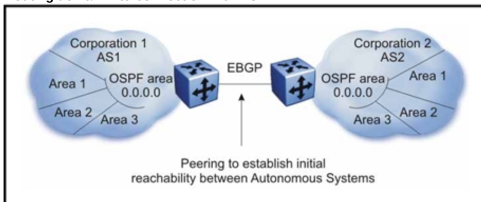
Figure 56 Routing domain interconnection with BGP
