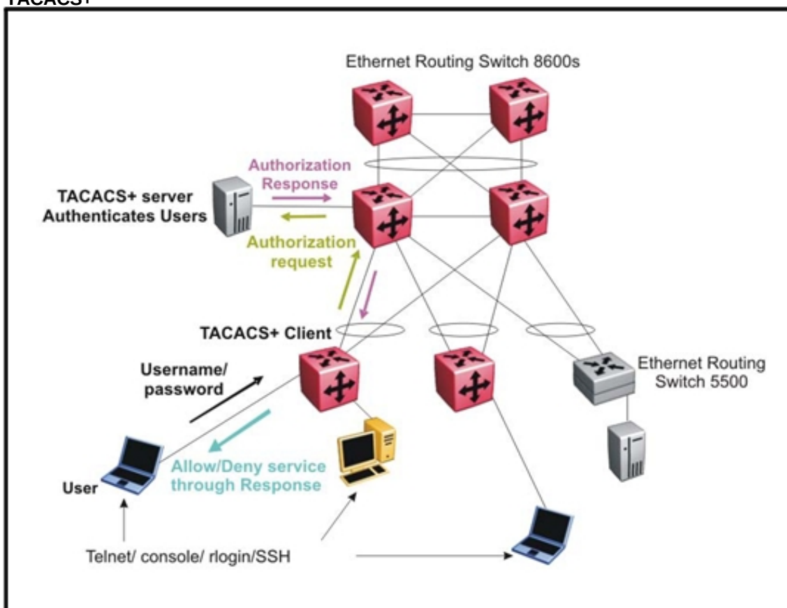
Figure 136 TACACS+
