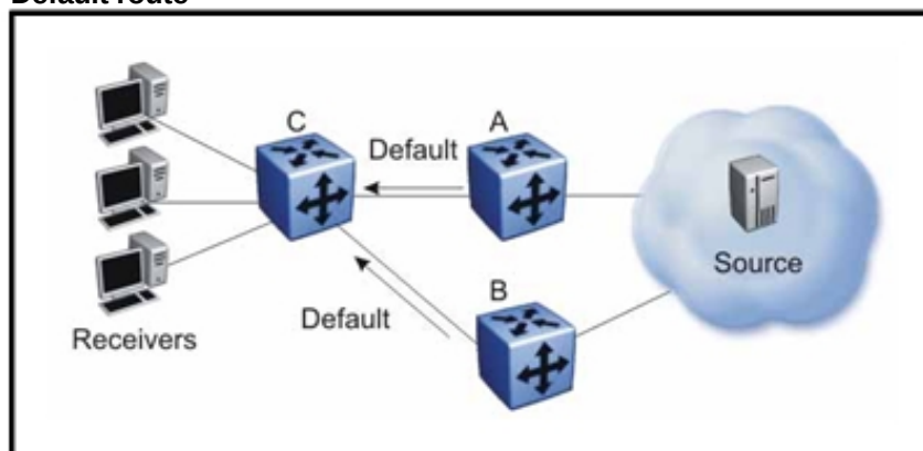
Figure 81 Default route
