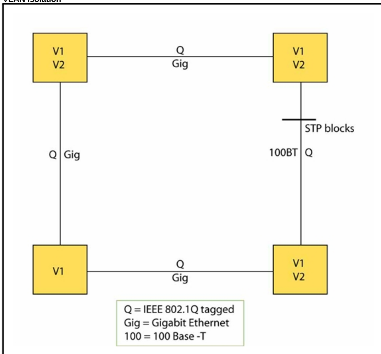
Figure 37 VLAN isolation
