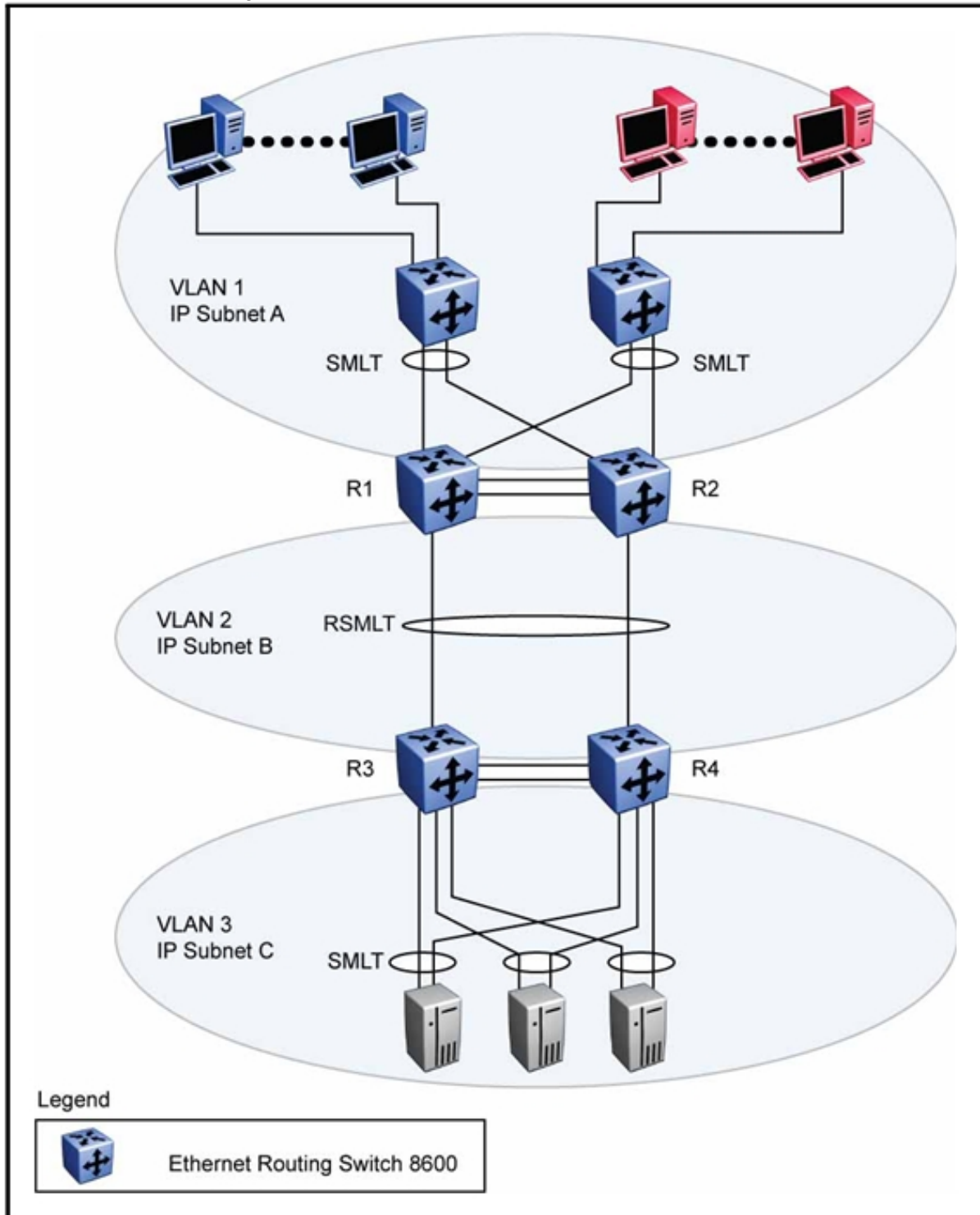
Figure 26 SMLT and RSMIT in Layer 3 environments
