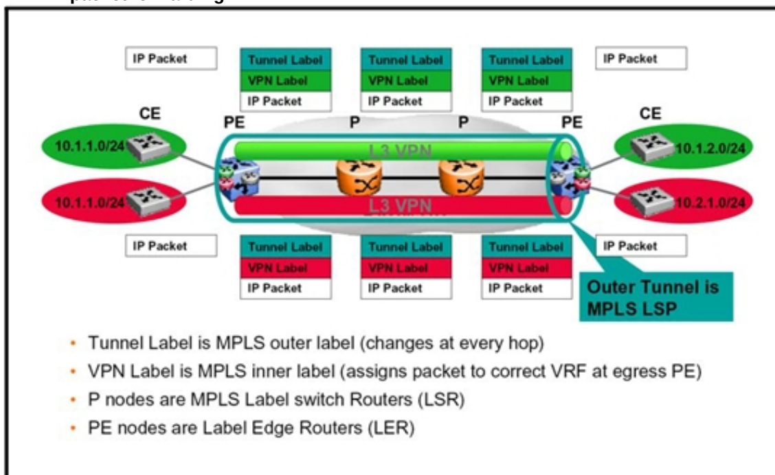
Figure 100 IP VPN packet forwarding
