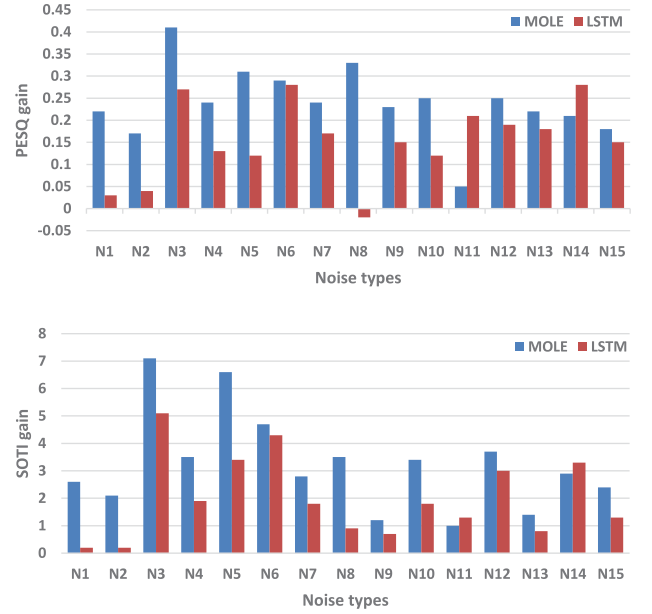
Fig. 4. Average PESQ/STOI gains of the MOLE and LSTM approaches compared with the DNN approach among 15 unseen noise types across all SNR levels.
