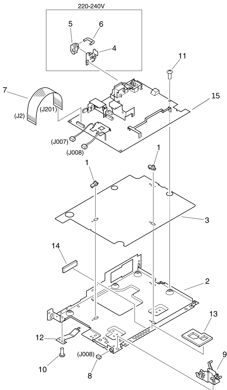
Figure 95. Electrical components
