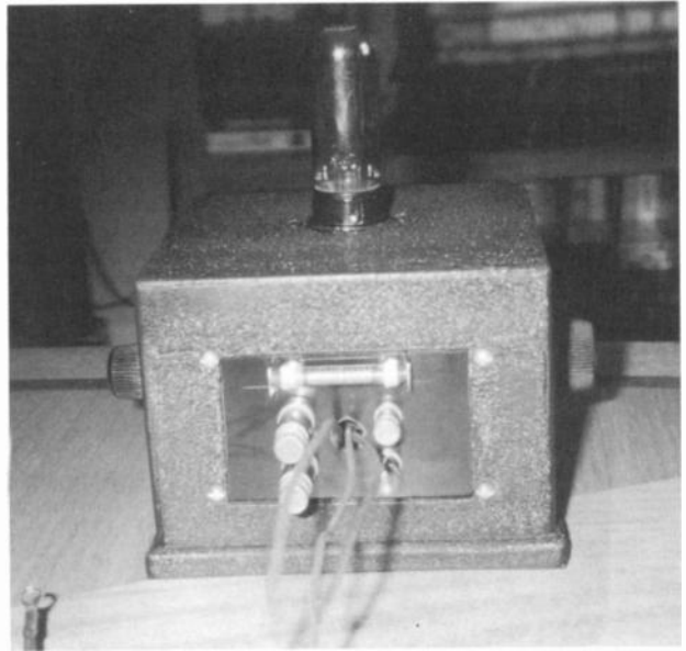
Figure 6. A rear view of the completed radio showing the Bakelite panel and its components.
