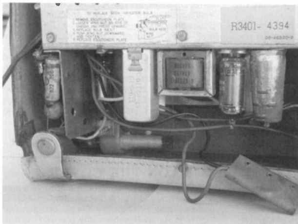
Figure 2. An interior view of the Prospector's inverted chassis and Geiger-Muller tube shown horizontally at the bottom.
