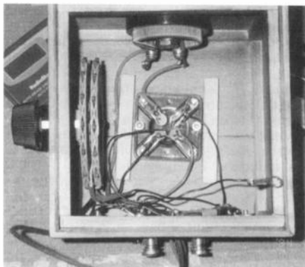
Figure 4. An underside view of the radio before installation of the tuning capacitor.
