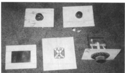
Figure 2. The wood cabinet panels with all components mounted and the rear panel cut to accept the Bakelite panel.
