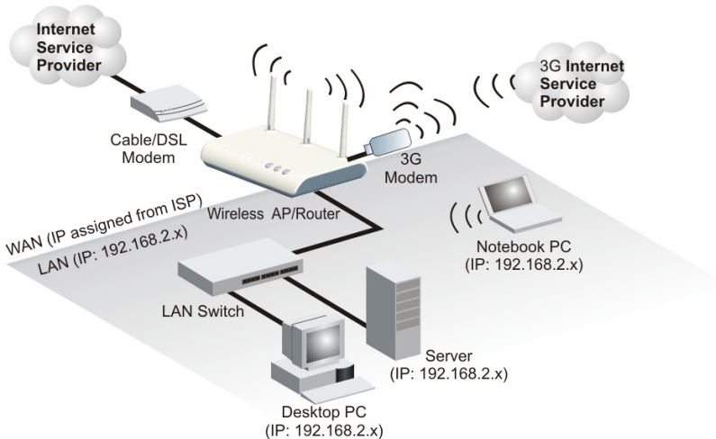
Figure 3-1. Operating as an Internet Gateway Router
