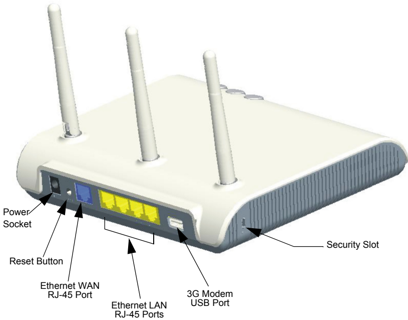
Figure 1-1. Rear Panel
