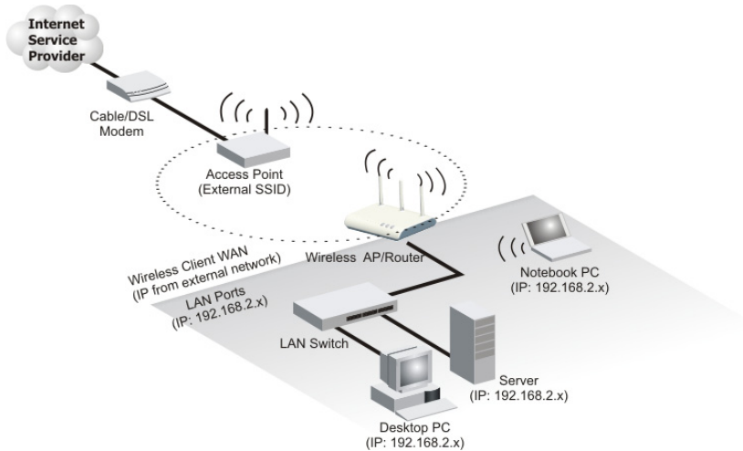
Figure 3-3. Operating with a Wireless Client WAN Connection
