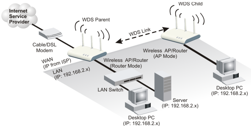
Figure 3-4. Operating as a Wireless Bridge
