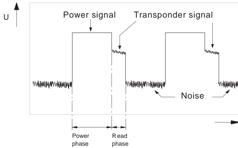
Figure 21. Monitored Signal Voltage at the Spectrum Analyser (Time Domain Mode)
