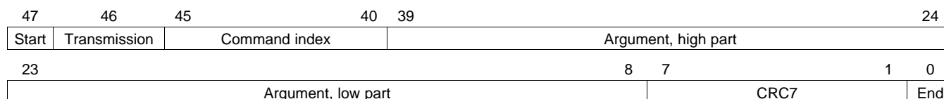
Figure 30. Command Format
