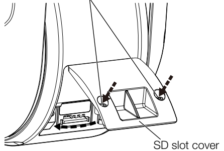
SD slot cover fixing screws
