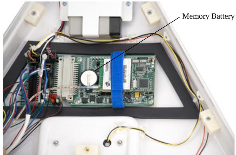
FIGURE 6-8. Memory battery inside TurfWeather station
