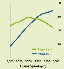
KAPPA 1.0 MPI ENGINE
