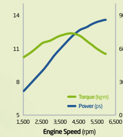
KAPPA 1.2 MPI ENGINE
