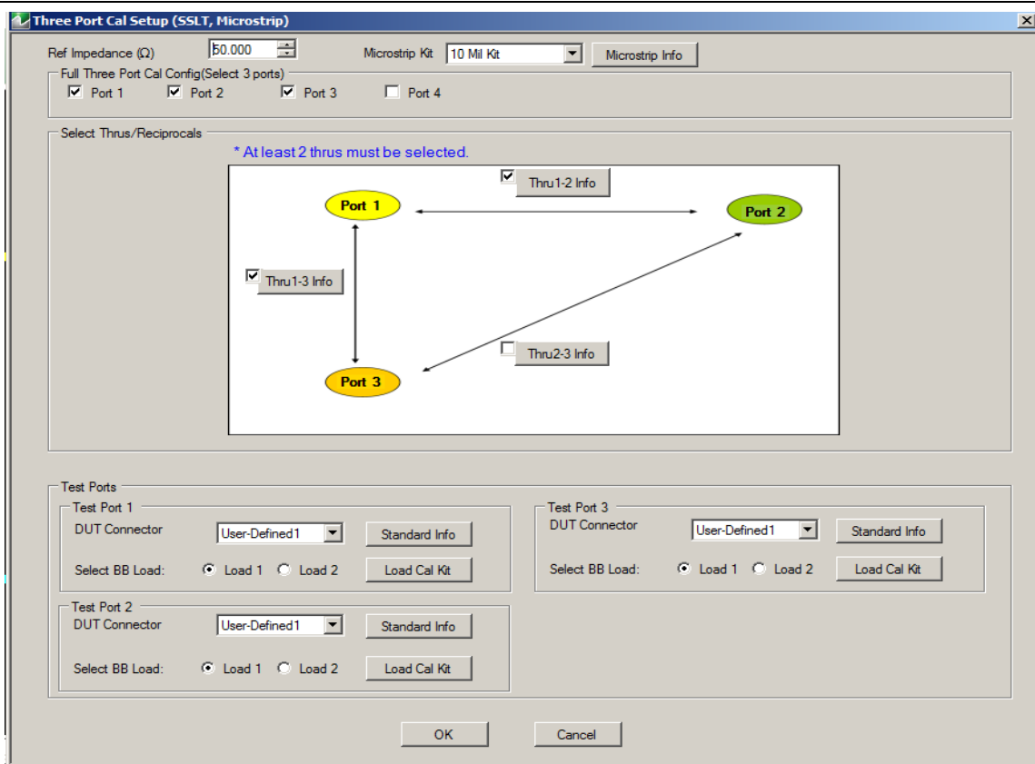
Figure 10-41. THREE PORT CAL SETUP (SSLT, MICROSTRIP) Dialog Box
