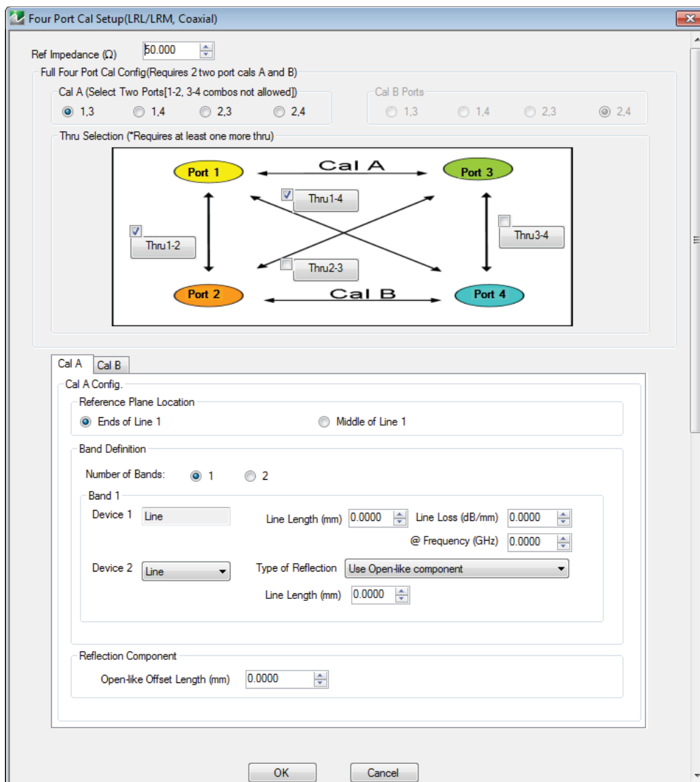
Figure 10-35. FOUR PORT CAL SETUP (LRL/LRM, COAXIAL) Dialog Box
