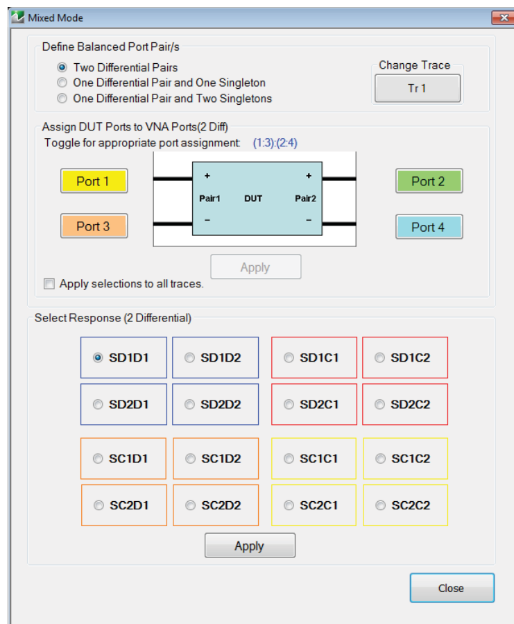
Figure 16-9. MIXED MODE Dialog Box - Two Differential Pairs
