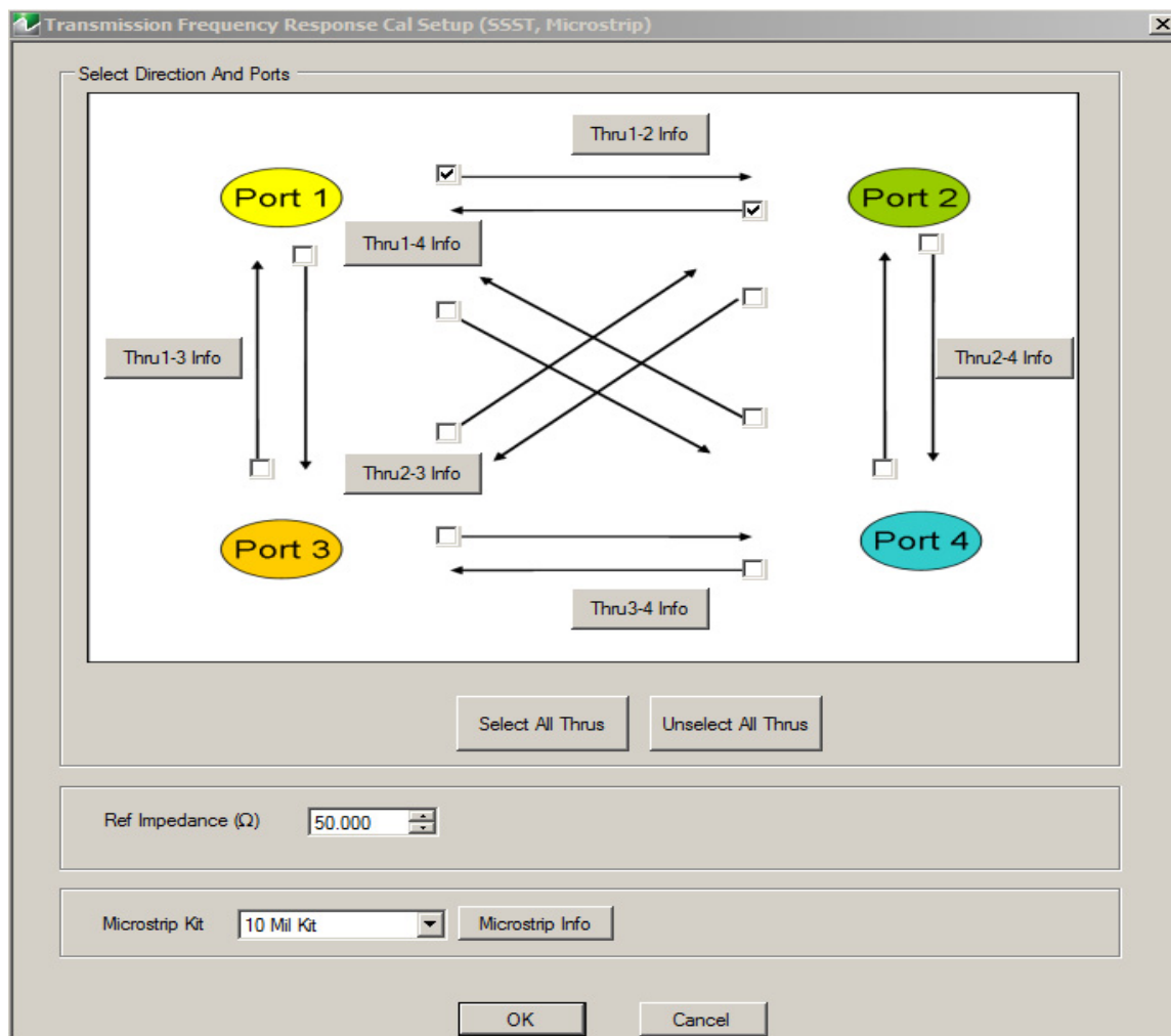
Figure 10-59. TRANS. FREQ. RESP. CAL SETUP (SSST, MICROSTRIP) Dialog Box
