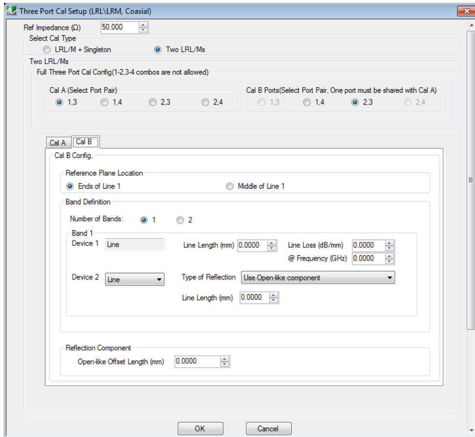
Figure 10-45. THREE PORT CAL SETUP (LRL/LRM, COAXIAL) Dialog Box - Cal B Tab
