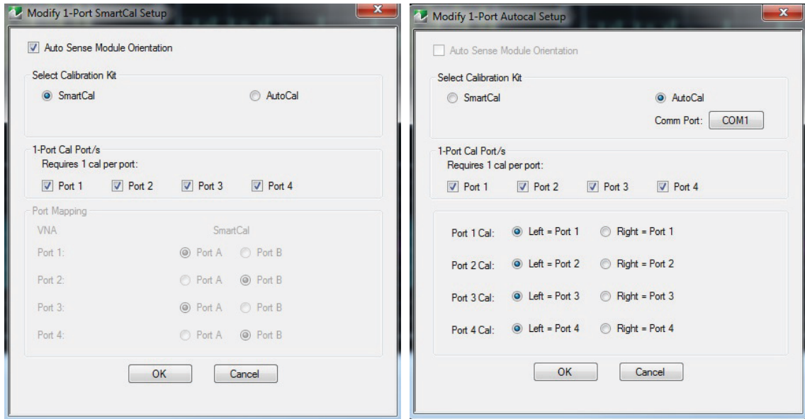
Figure 10-23. MODIFY 1-PORT AUTOCAL/SMARTCAL SETUP Dialog Box - 4-Port VNAs
