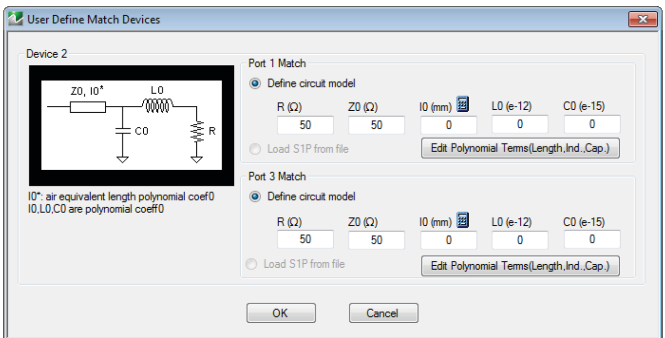
Figure 10-71. USER DEFINED MATCH DEVICES Dialog Box - LRL/LRM
