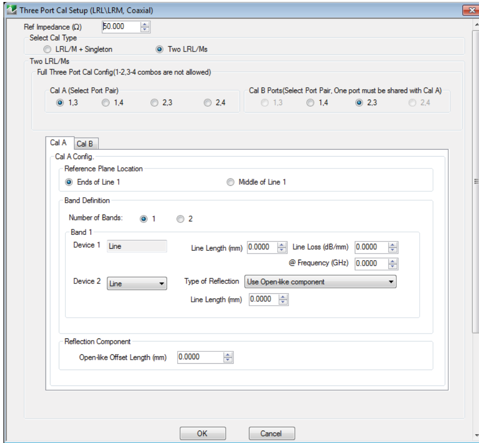
Figure 10-44. THREE PORT CAL SETUP (LRL/LRM, COAXIAL) Dialog Box - Cal A Tab
