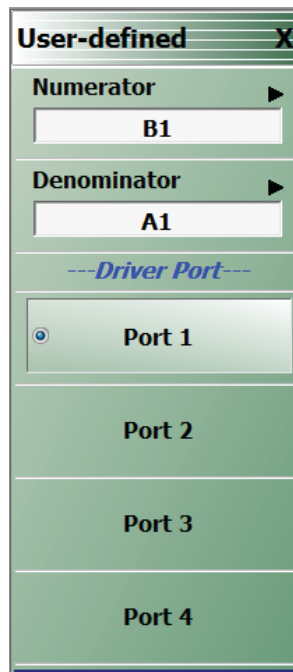
Figure 16-6. USER DEFINED Menu - 4-Port VNAs
