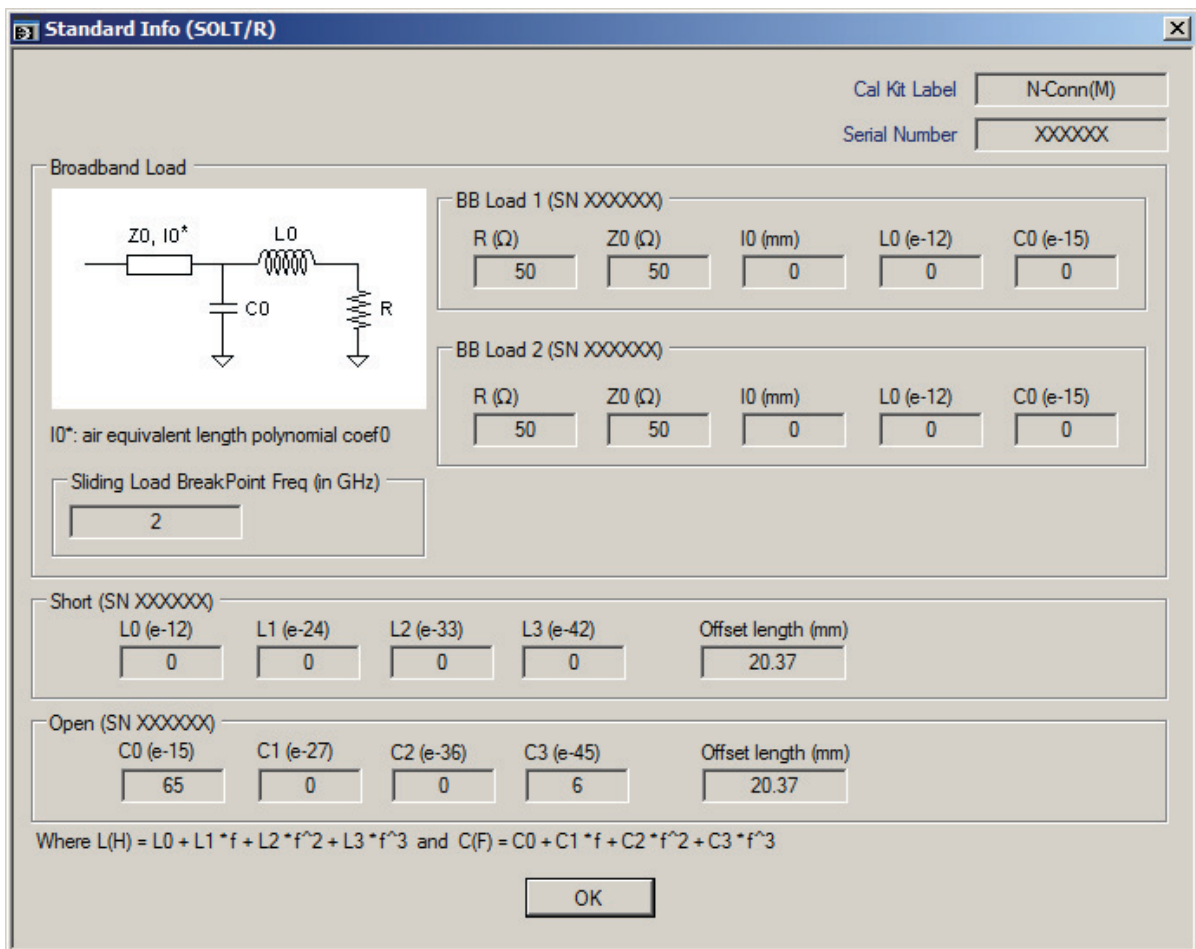
Figure 9-45. STANDARD INFO (SOLT/R) Dialog Box
