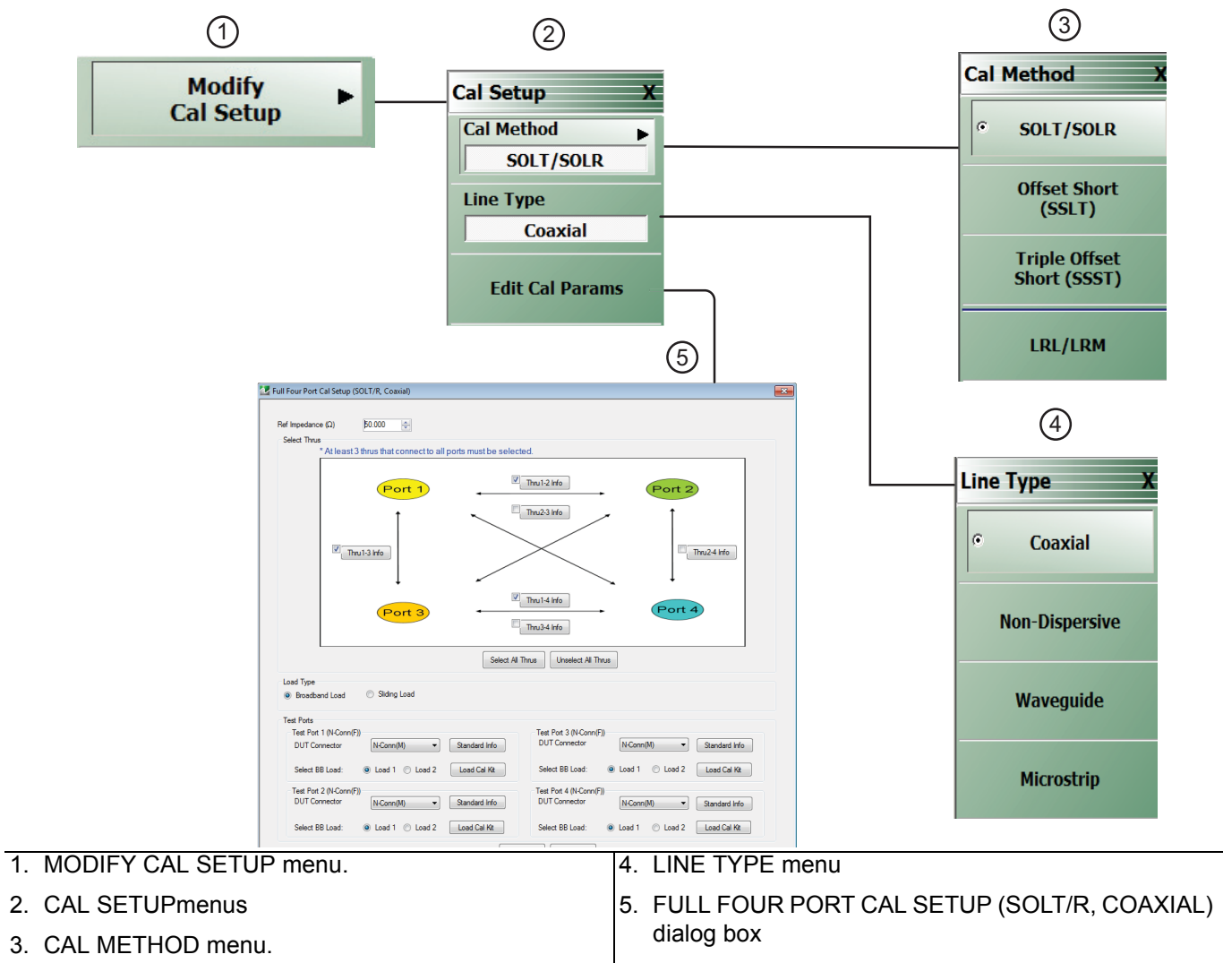
Figure 10-25. Manual Calibration Setup Menus - 4-Port VNAs - Sheet 2
