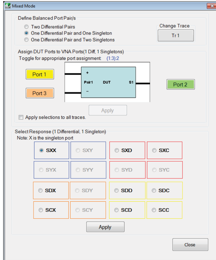
Figure 16-10. MIXED MODE Dialog Box - One Differential Pair and One Singleton - 4-Port VNAs
