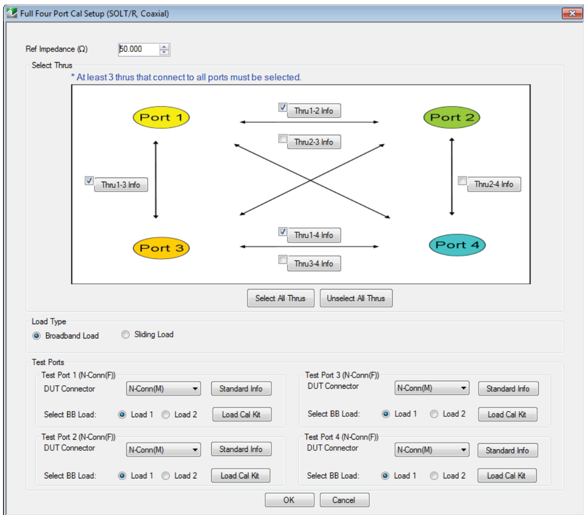
Figure 10-31. FULL FOUR PORT CAL SETUP (SOLT/R, COAXIAL) Dialog Box
