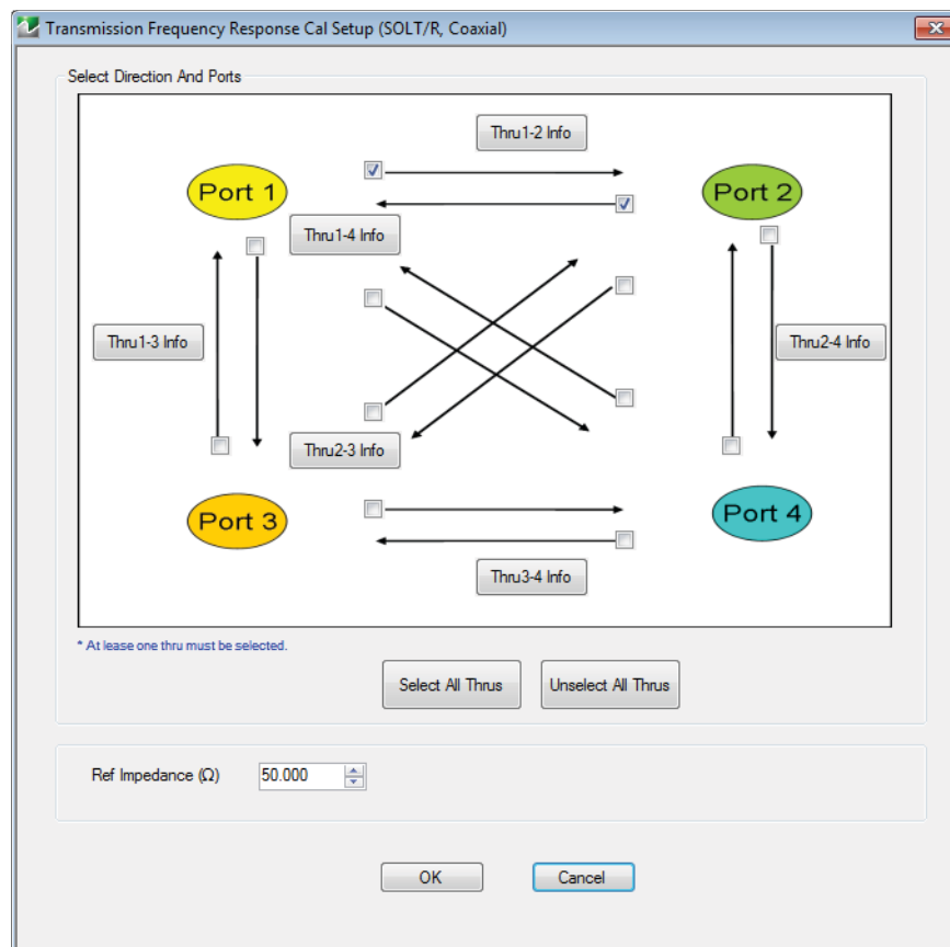
Figure 10-57. TRANSMISSION FREQ. RESPONSE CAL SETUP (SOLT/R, COAXIAL) Dialog Box
