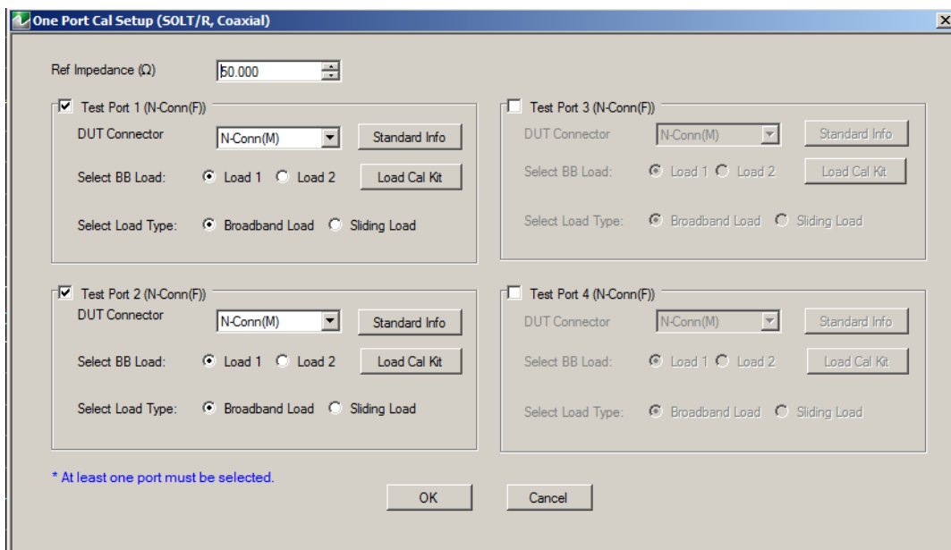
Figure 9-38. ONE-PORT CAL SETUP (SSLT, COAXIAL) Dialog Box
