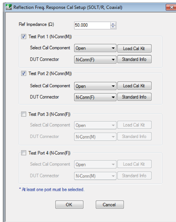
Figure 10-61. REFLECTION FREQ. RESPONSE. CAL SETUP (SOLT/R, COAXIAL) Dialog Box
