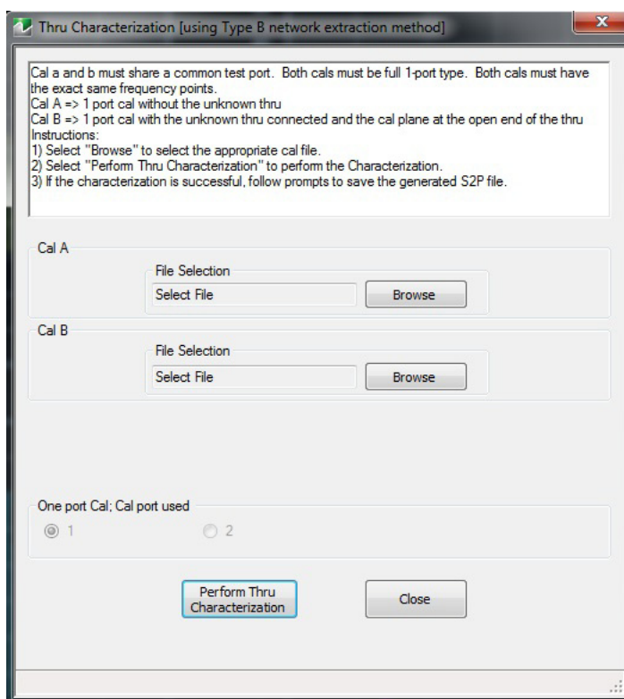
Figure 9-15. THRU CHARACTERIZATION Dialog Box
