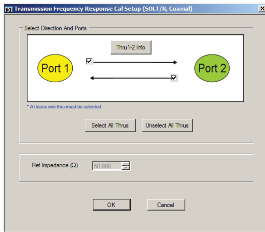
Figure 9-41. TRANSMISSION FREQUENCY RESPONSE CAL SETUP (SOLT/R, COAXIAL) Dialog Box
