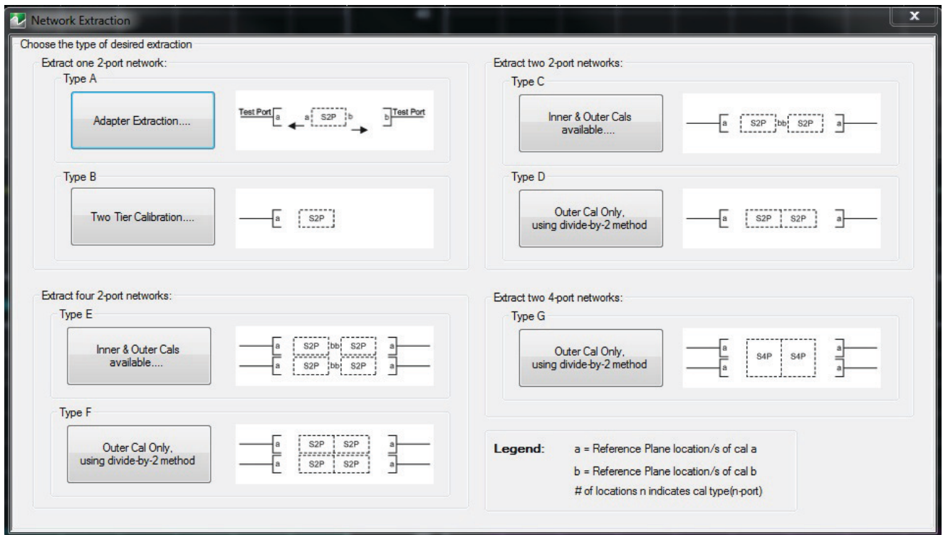
NETWORK EXTRACTION Dialog Box – Choose the type of desired extraction from the buttons below:
