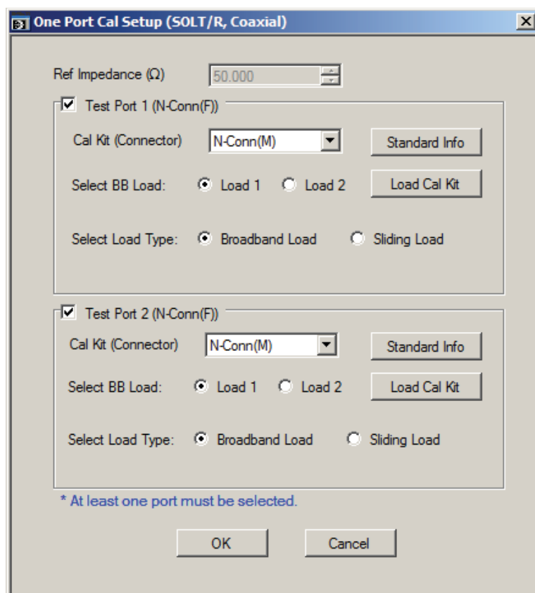
Figure 9-37. ONE-PORT CAL SETUP (SOLT/R, COAXIAL) Dialog Box
