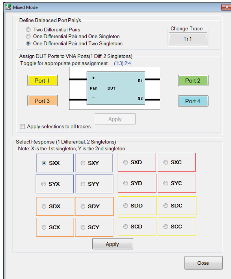
Figure 16-11. MIXED MODE Dialog Box - One Differential Pair and Two Singletons - 4-Port VNAs
