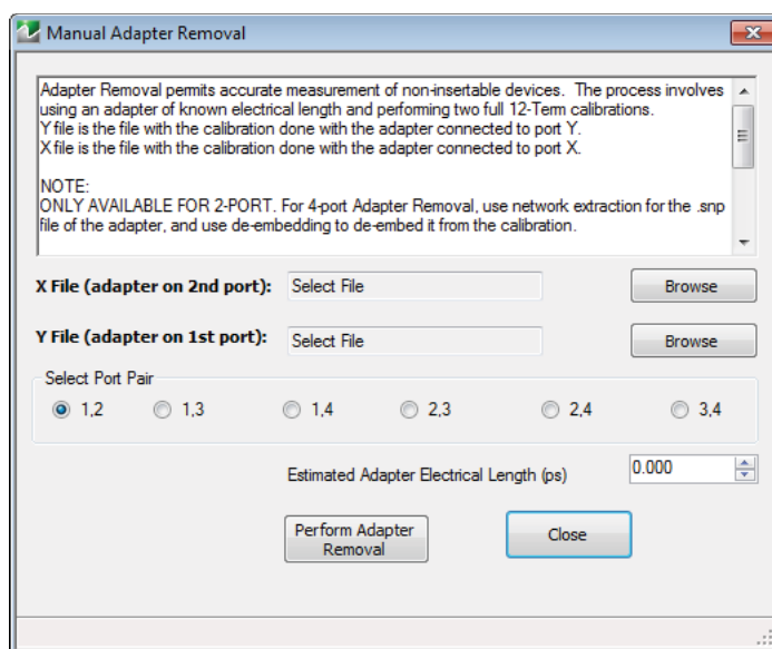
Figure 9-13. MANUAL ADAPTER REMOVAL Dialog Box
