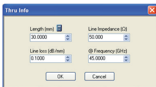
Figure 9-46. THRU INFO Dialog Box - AutoCal Two Port Calibration
