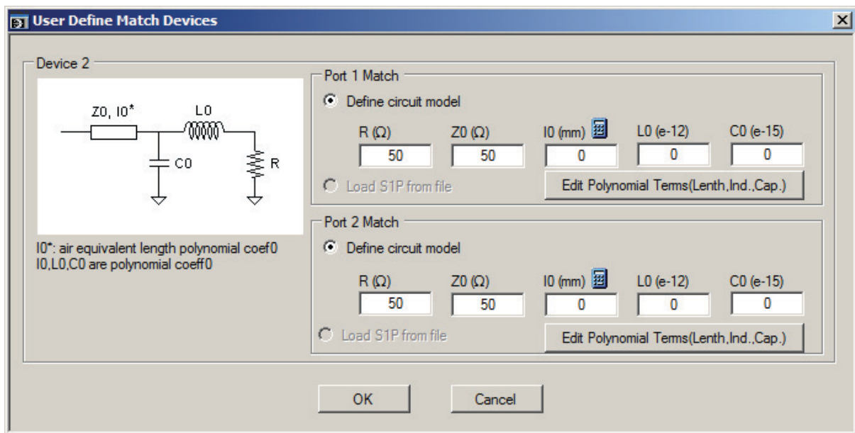
Figure 9-47. USER DEFINED MATCH DEVICES Dialog Box - 2-Port VNAs
