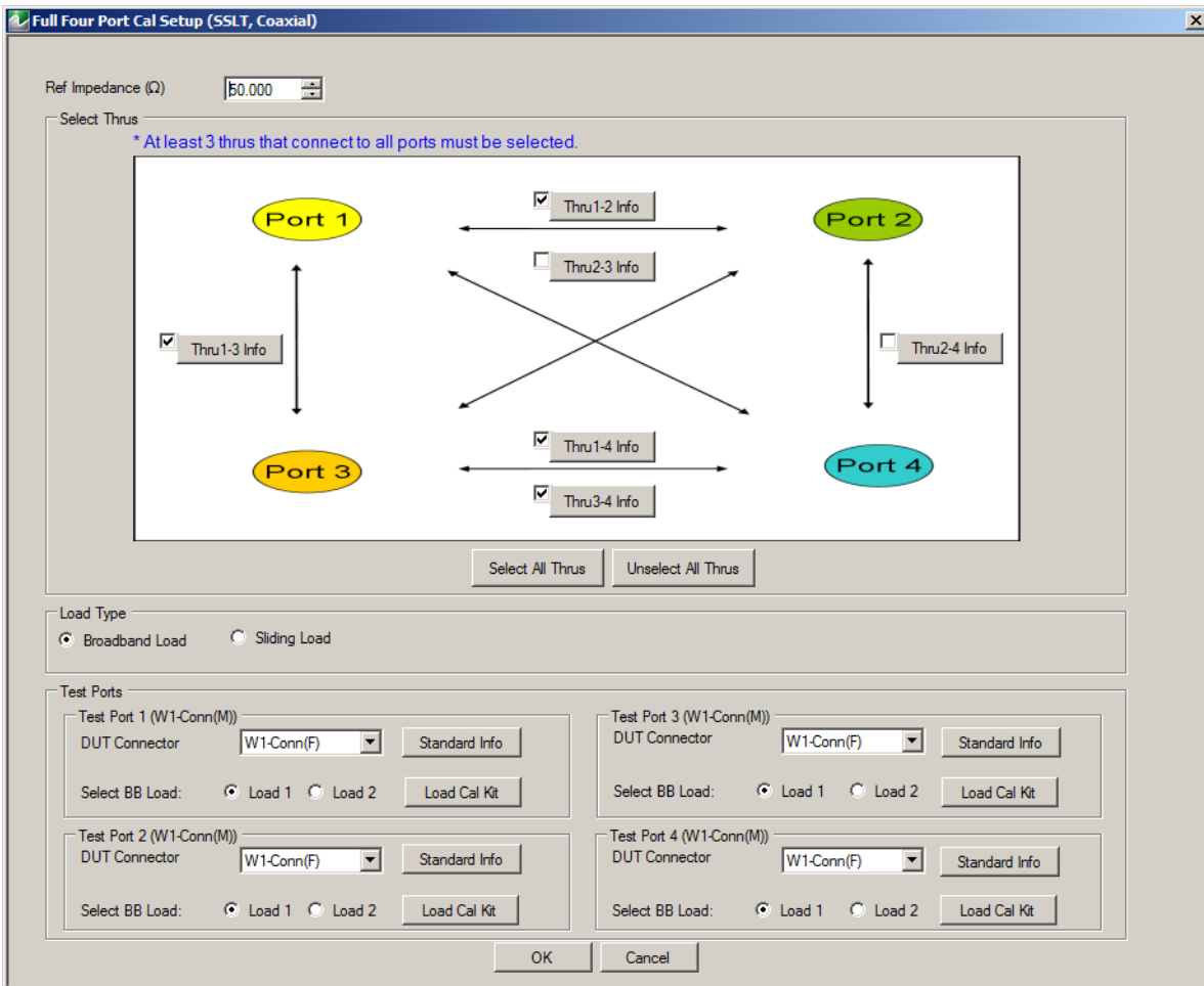
Figure 10-32. FULL FOUR PORT CAL SETUP (SSLT, COAXIAL) Dialog Box
