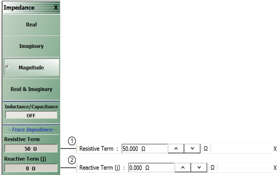
Figure 17-3. IMPEDANCE Menu
