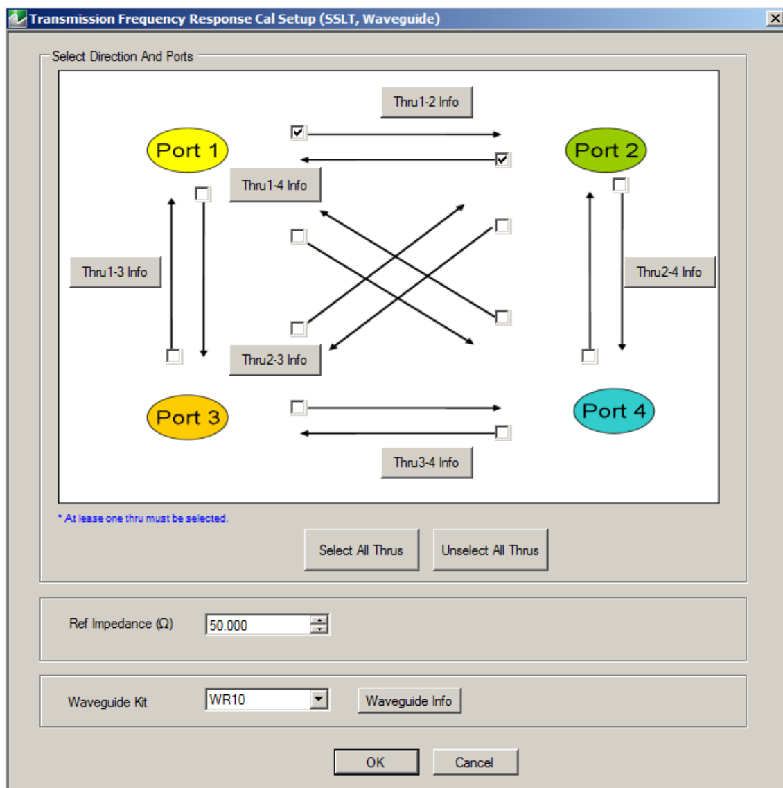
Figure 10-58. TRANS. FREQ. RESP. CAL SETUP (SSLT, WAVEGUIDE) Dialog Box
