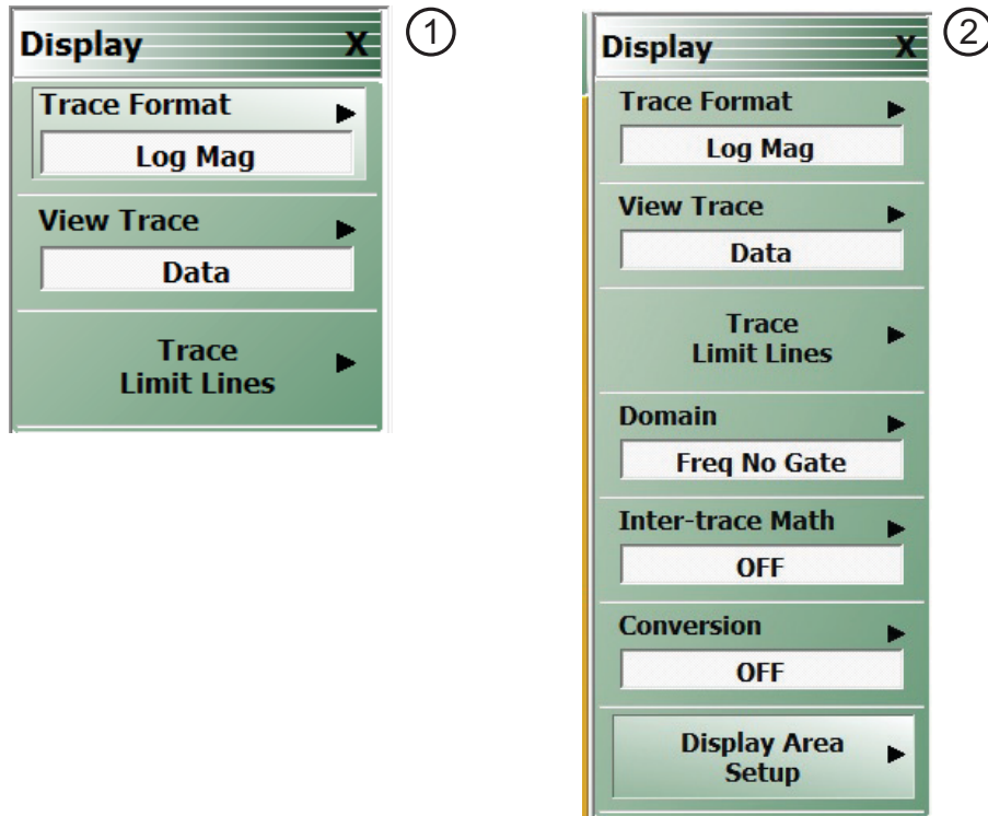
Figure 17-1. DISPLAY Menu
