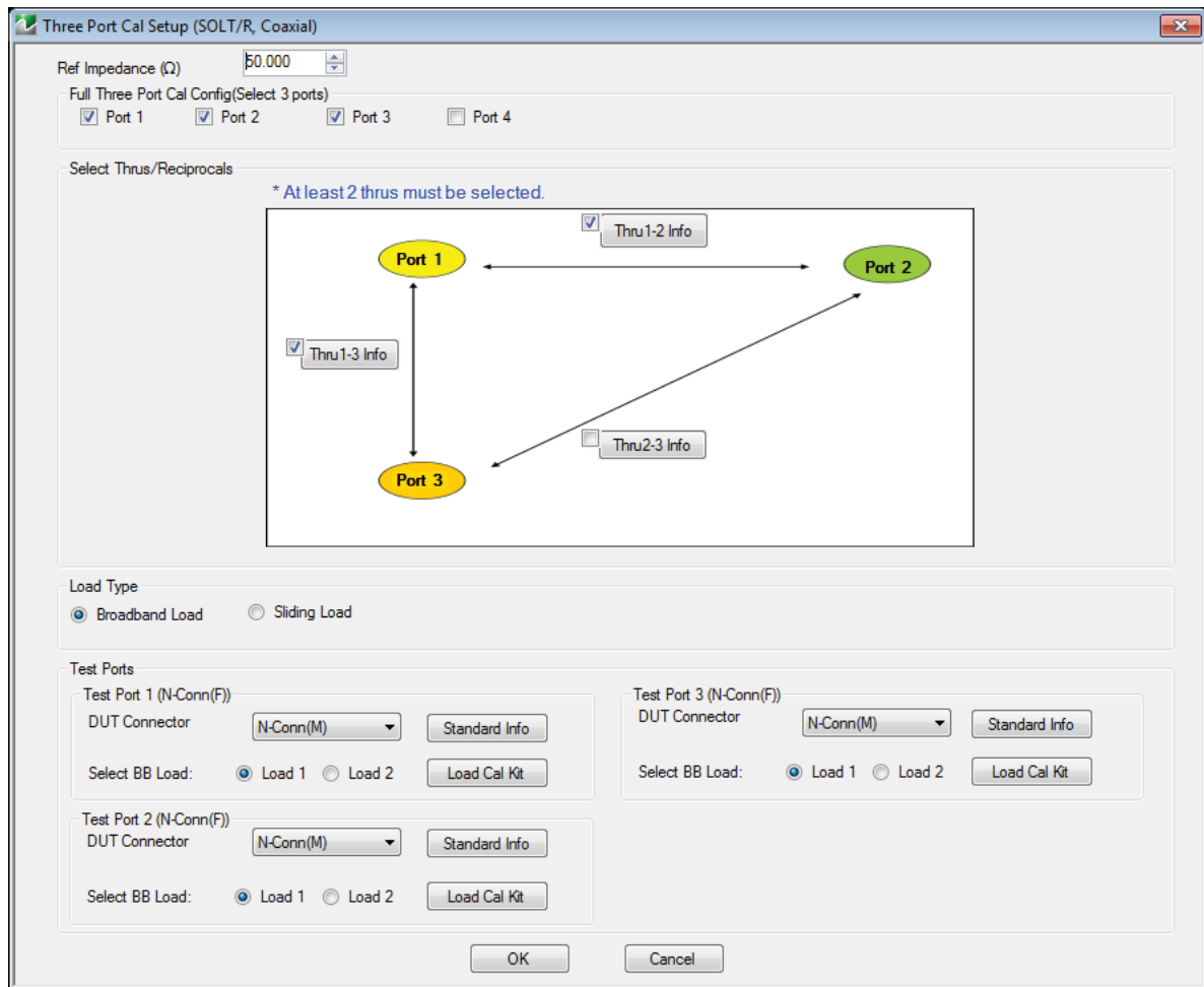
Figure 10-43. THREE PORT CAL SETUP (SOLT/R, COAXIAL) Dialog Box
