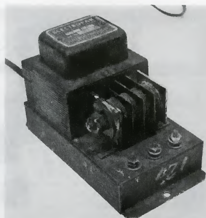
Figure 3. A power supply that utilizes a magnesium copper sulfide rectifier.
