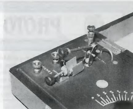
Figure 5. Close-up of the detector showing rear-pivoted detector arm and crystal holder with cover.
