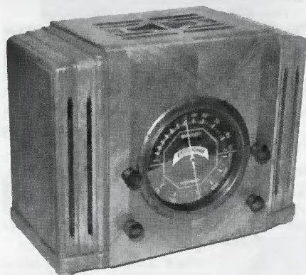
SILVERTONE UNKNOWN — This remarkably well-preserved AC set was unearthed at a North Carolina antique shop in June 1996. Resembling a 1930s era console with the bottom sawed off (actually, the speaker is built-in to the top), it's a strong performer on both the AM (550-1700 kHz) and shortwave (2.5-7 MHz) bands, yet uses only 5 tubes (Types 42, 75, 80, 6D6, and 6A7). The bottom of the wooden case is stamped "MAR 24, 1936." The same set is pictured in Evolution of the Radio, Volume 2 , and is similarly identified. Can anyone tell me the model number and year of production? (Douglas D. Fox — St. Charles, IL)
