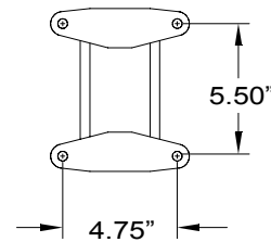
MOUNTING DIMENSIONS
