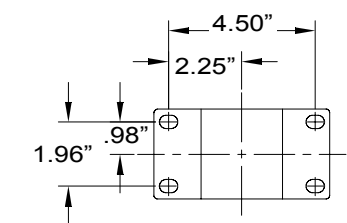
MOUNTING DIMENSIONS
