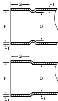
Female End
