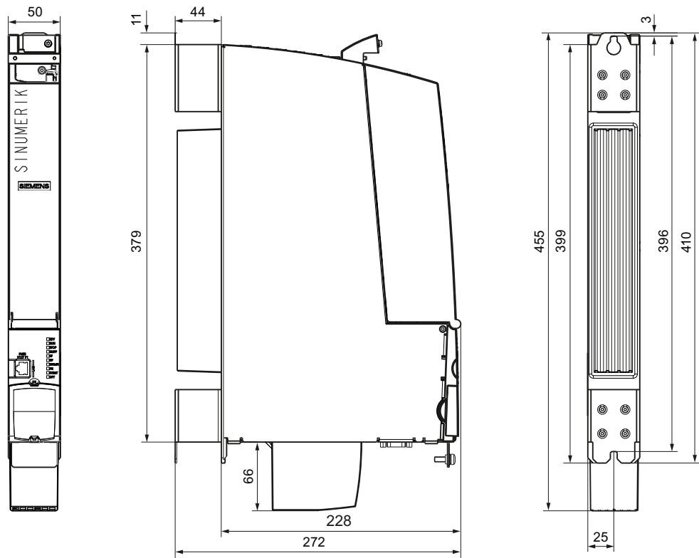
Figure 5-1 Dimension drawing NCU 720.3 PN ( ... -0AA1) and NCU 730.3 PN; dimensions in mm
