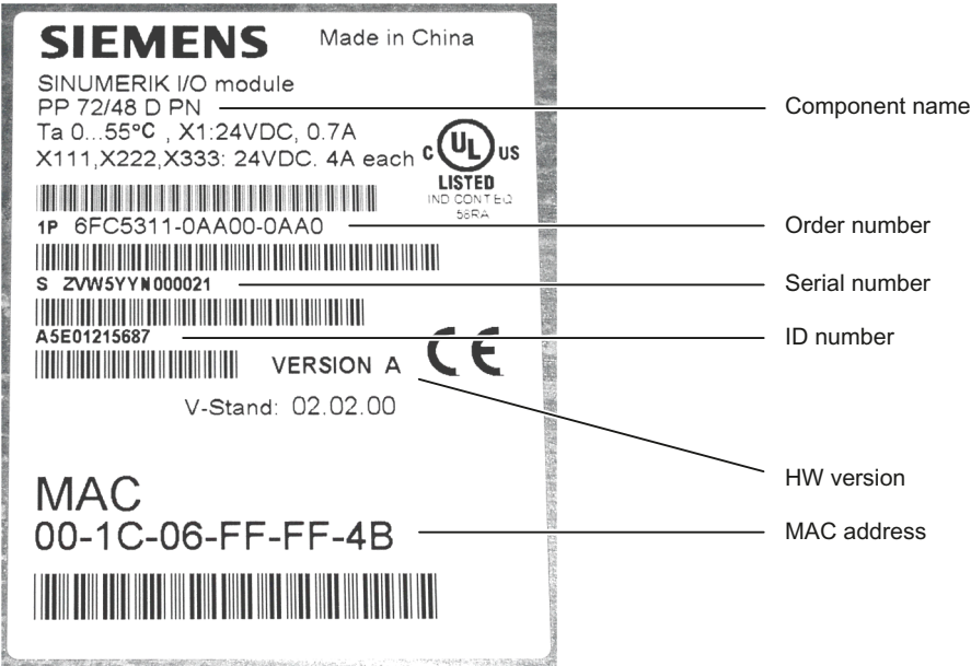
Figure 9-8 PP 72/48D PN type plate
