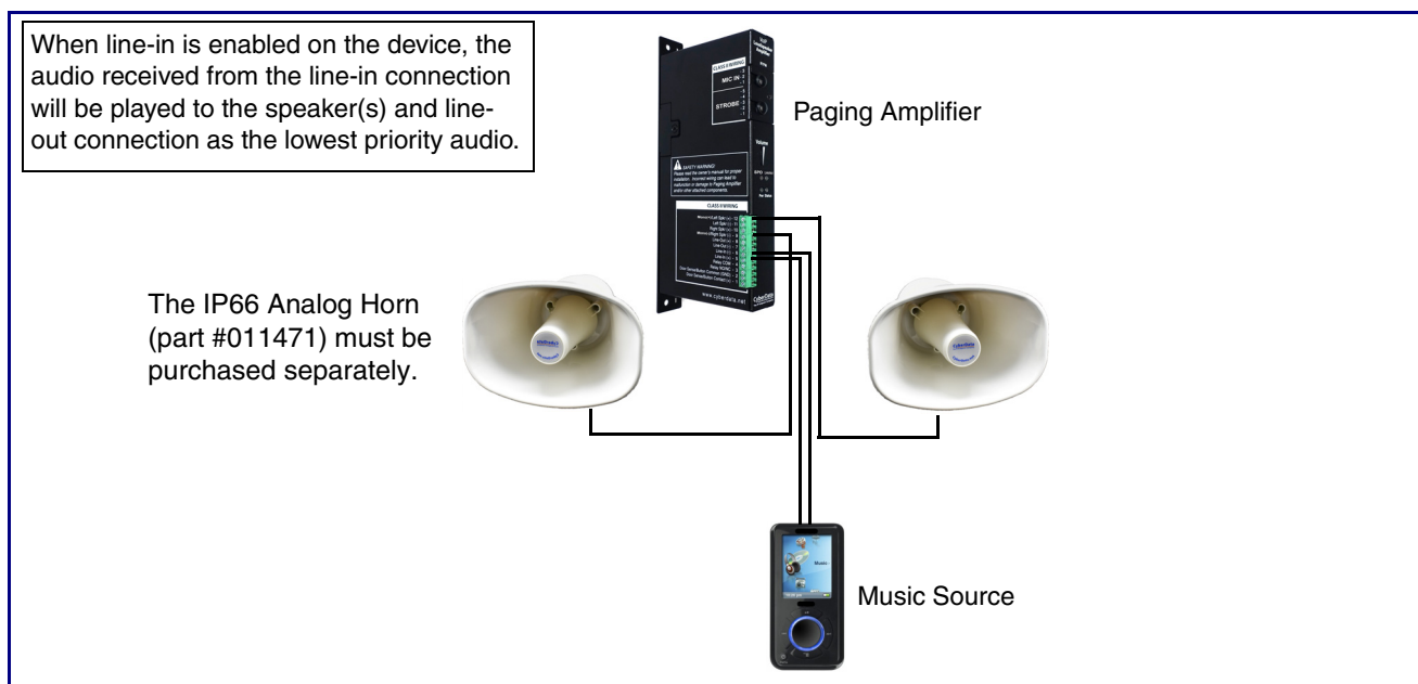
Figure 2-10. Line-In Connection
