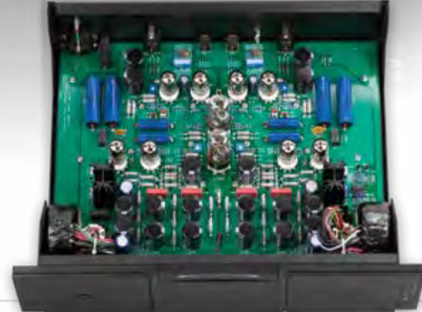
BAT VK-P6 Phonostage $3,495
